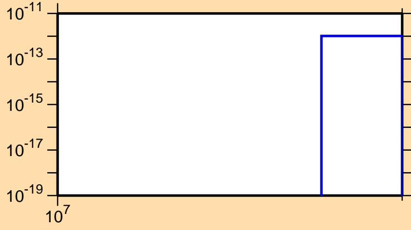
\sigma vs. E for ^{148}\text{La} (mt 11)
