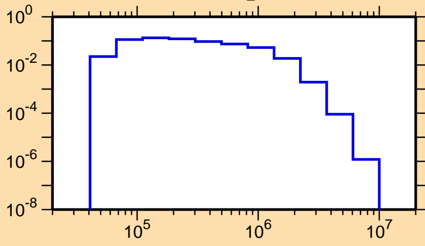
\sigma vs. E for ^{148}\text{La}(n,n_2)
