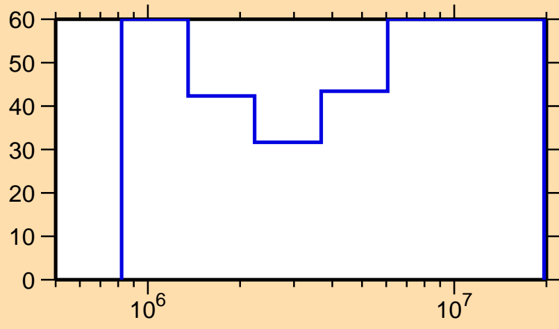
\Delta\sigma/\sigma vs. E for ^{148}\text{La}(n,n\text{cont.})
