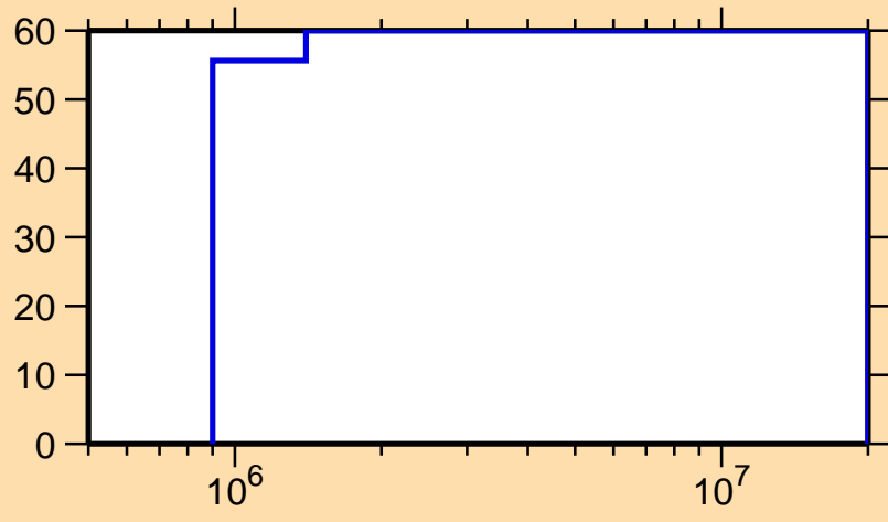
\Delta\sigma/\sigma vs. E for ^{148}\text{La}(n,n_1)
