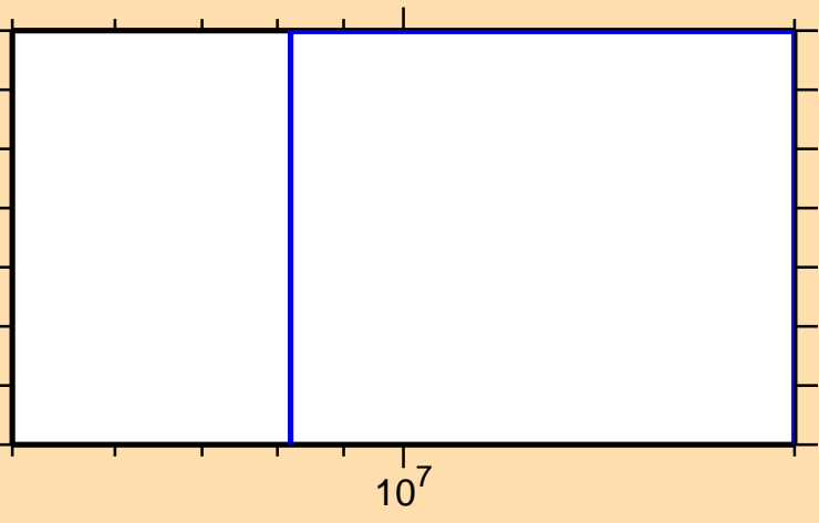
\sigma vs. E for ^{148}\text{La}(n,n\alpha)
