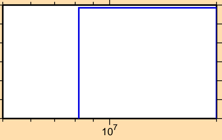
\sigma vs. E for ^{148}\text{La}(n,\text{nd})
