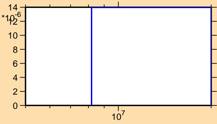
\sigma vs. E for ^{148}\text{La}(n,n\alpha)
