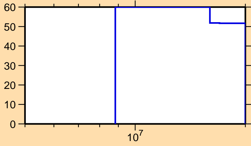
\Delta\sigma/\sigma vs. E for ^{149}\text{La}(n,p)
