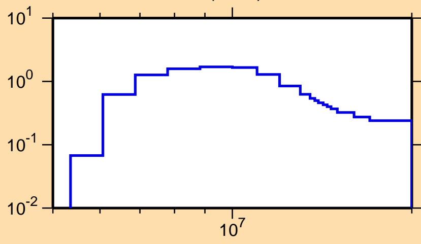
\sigma vs. E for ^{149}\text{La}(n,2n)
