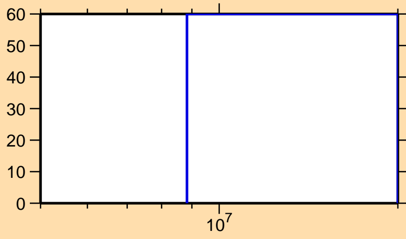
\Delta\sigma/\sigma vs. E for ^{149}\text{La}(n,\gamma)
