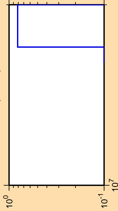
\Delta\sigma/\sigma vs. E for ^{149}\text{La}(n,3n\alpha)
