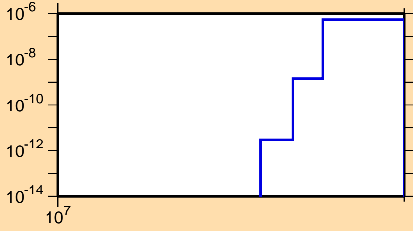
\sigma vs. E for ^{149}\text{La}(n,\text{nd})
