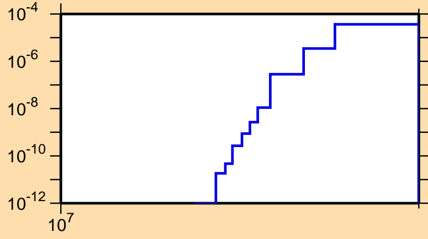
\sigma vs. E for ^{149}\text{La}(n,nt)
