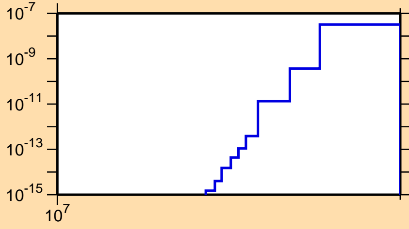
\sigma vs. E for ^{149}\text{La}(n,2n\alpha)
