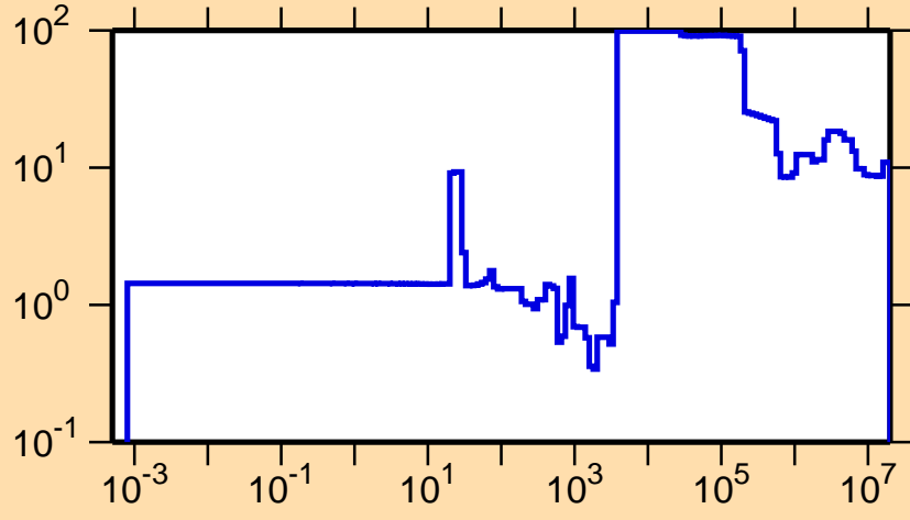
\Delta\sigma/\sigma vs. E for ^{149}\text{La}(n,\text{el.})
