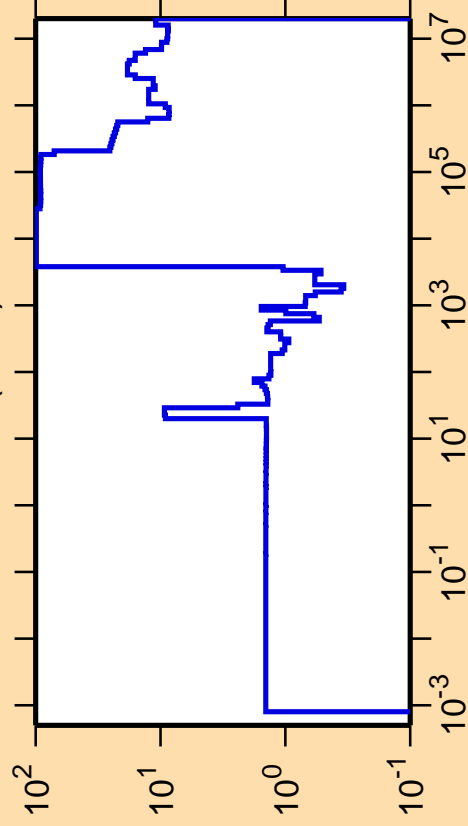
\Delta\sigma/\sigma vs. E for ^{149}\text{La}(n,\text{el.})
