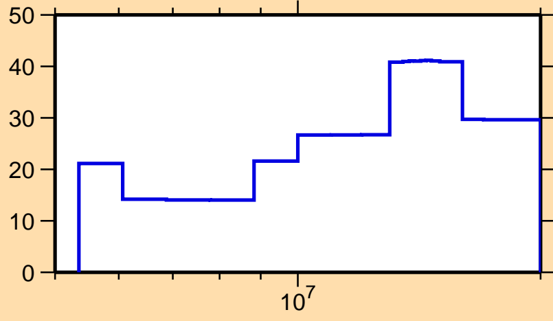
\Delta\sigma/\sigma vs. E for ^{149}\text{La}(n,2n)
