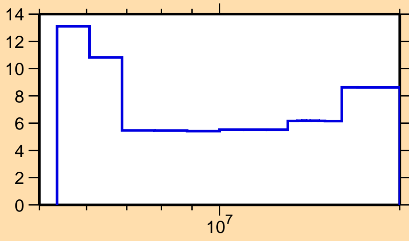
\Delta\sigma/\sigma vs. E for ^{149}\text{La}(n,\text{tot.})
