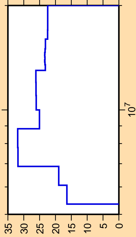
\Delta\sigma/\sigma vs. E for ^{149}\text{La}(n,n\text{cont.})
