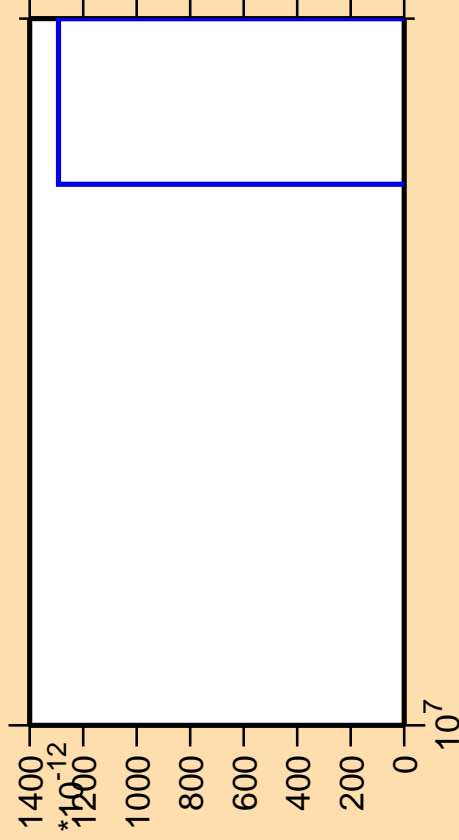
\Delta\sigma/\sigma vs. E for ^{149}\text{La} (mt 42)
