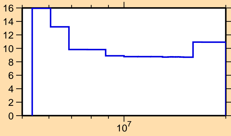
\Delta\sigma/\sigma vs. E for ^{149}\text{La}(n,\text{el.})
