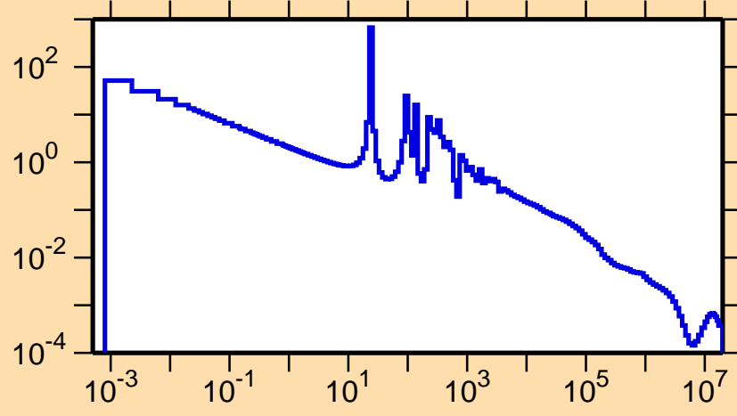
\sigma vs. E for ^{149}\text{La}(n,\gamma)
