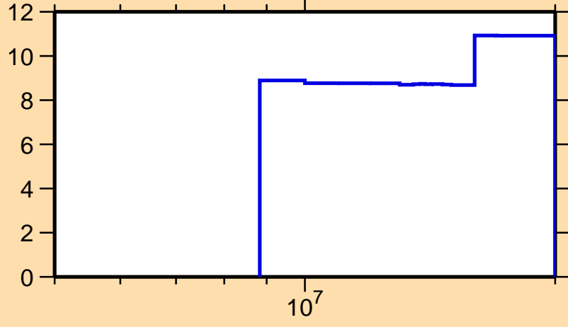
\Delta\sigma/\sigma vs. E for ^{149}\text{La}(n,el.)
