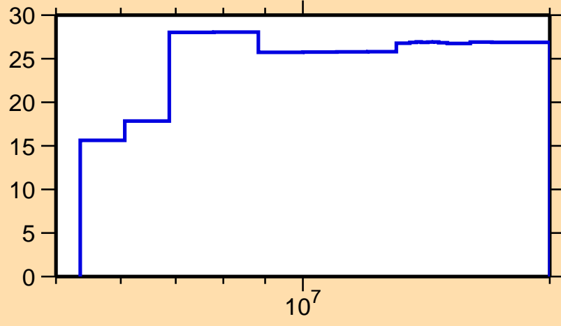
\Delta\sigma/\sigma vs. E for ^{149}\text{La}(n,\text{inel.})
