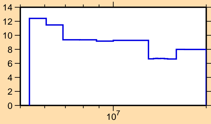
\Delta\sigma/\sigma vs. E for ^{149}\text{La}(n,\text{nonel.})
