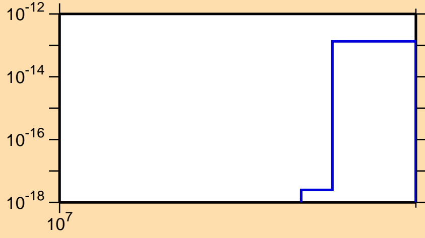
\sigma vs. E for ^{149}\text{La}(n,3n\alpha)
