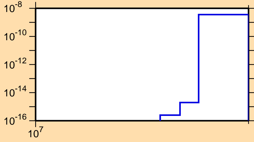
\sigma vs. E for ^{149}\text{La}(n,2np)
