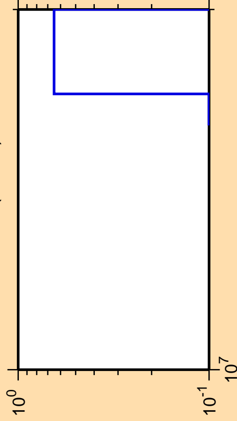
\Delta\sigma/\sigma vs. E for ^{149}\text{La} (mt 11)
