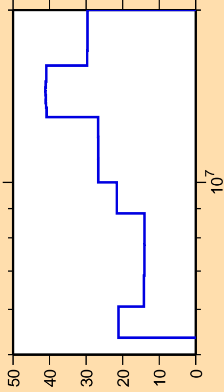
\Delta\sigma/\sigma vs. E for ^{149}\text{La}(n,2n)
