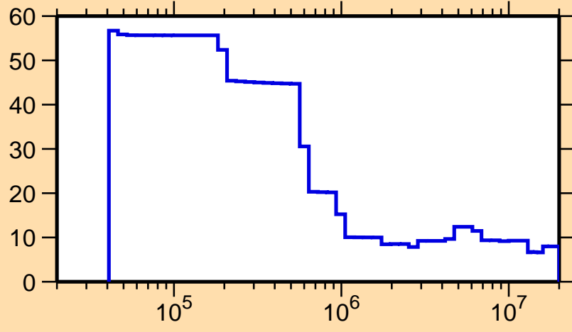
\Delta\sigma/\sigma vs. E for ^{149}\text{La}(n,\text{nonel.})
