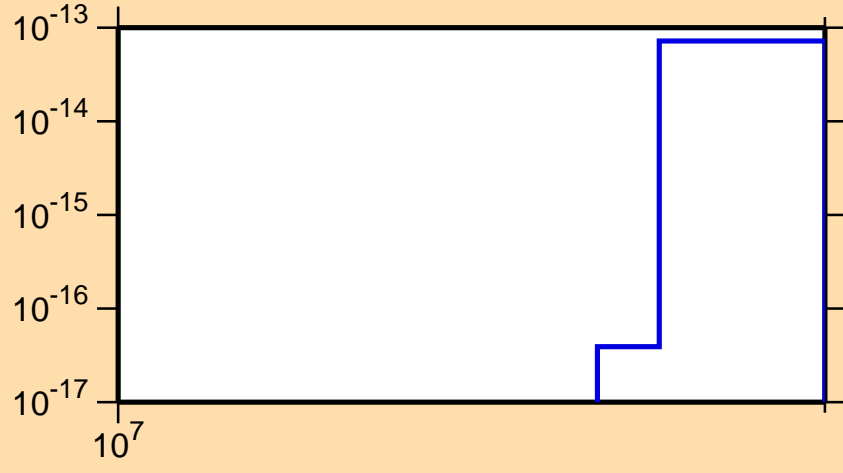
\sigma vs. E for ^{149}\text{La} (mt 11)
