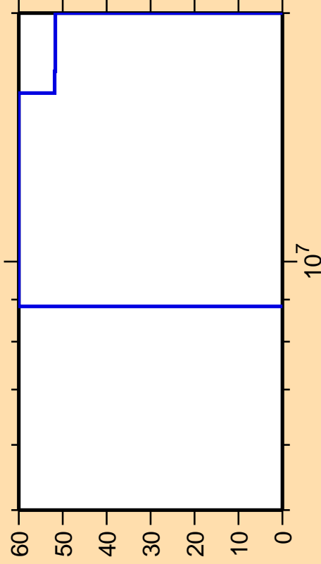
\Delta\sigma/\sigma vs. E for ^{149}\text{La}(n,p)
