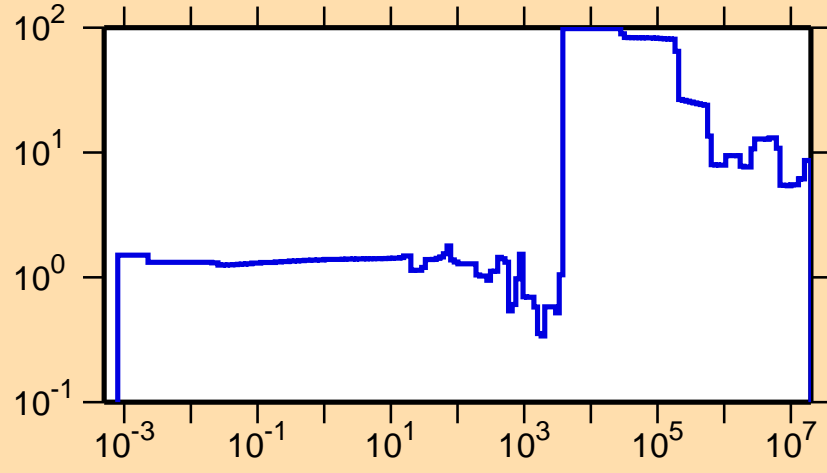
\Delta\sigma/\sigma vs. E for ^{149}\text{La}(n,\text{tot.})
