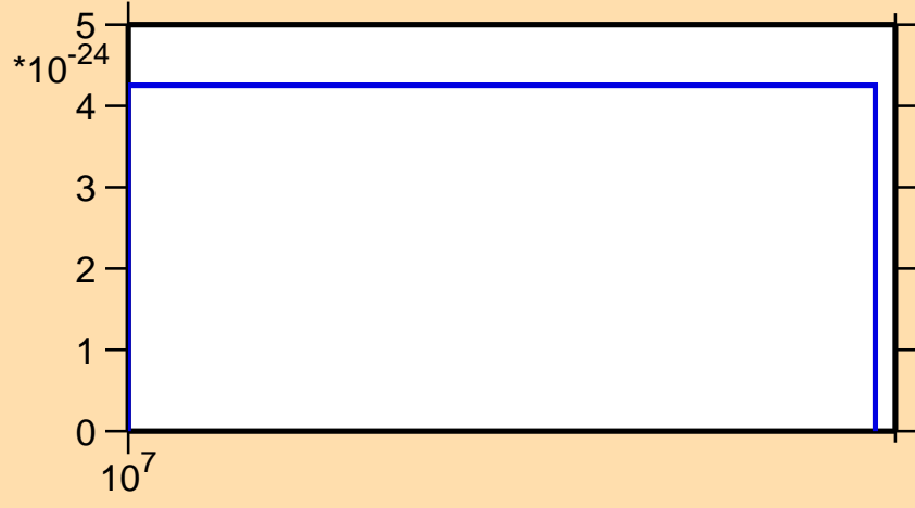
\sigma vs. E for ^{149}\text{La} (mt 42)
