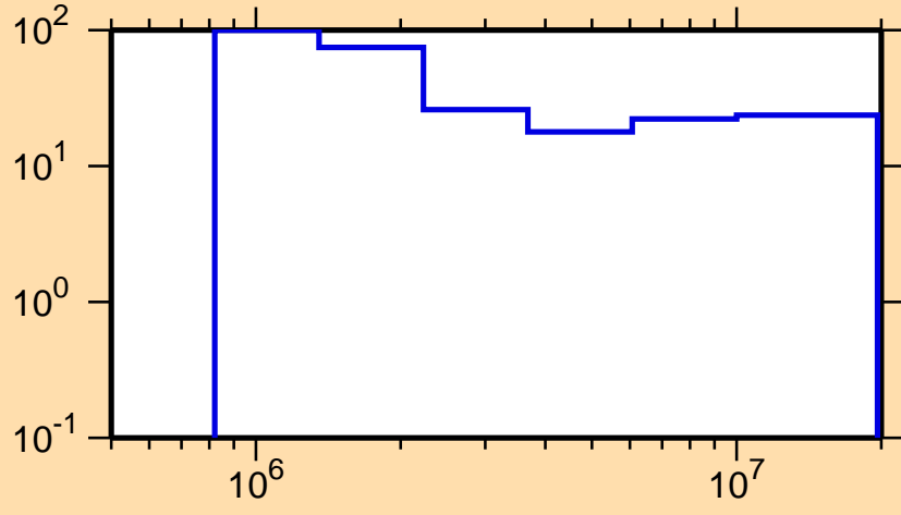
\Delta\sigma/\sigma vs. E for ^{149}\text{La}(n,n\text{cont.})
