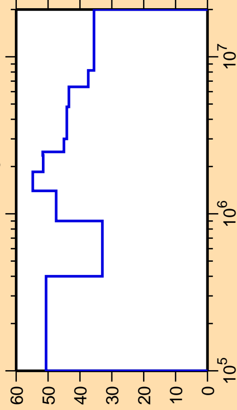
\Delta\sigma/\sigma vs. E for ^{149}\text{La}(n,n_3)
