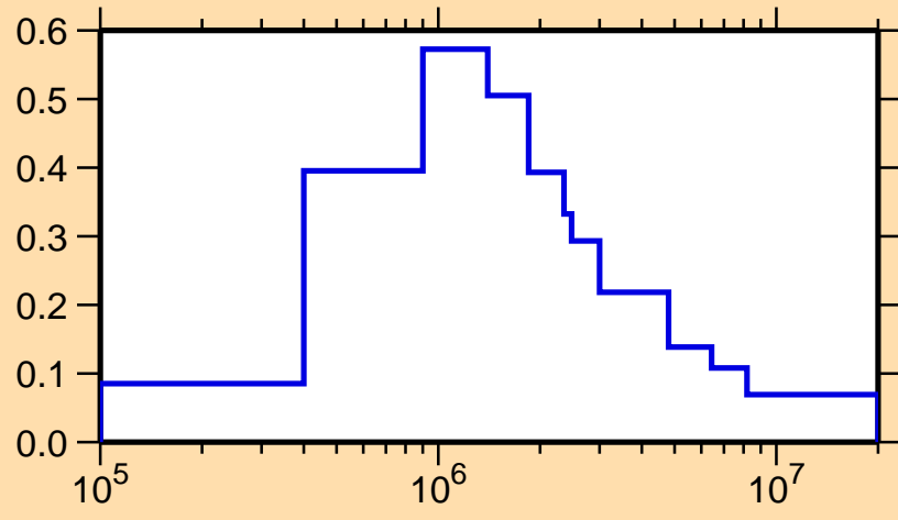
\sigma vs. E for ^{149}\text{La}(n,n_3)
