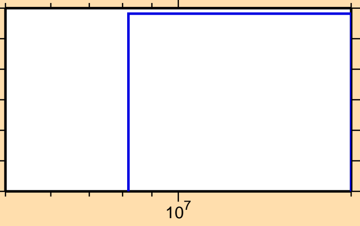
\sigma vs. E for ^{149}\text{La}(n,2np)
