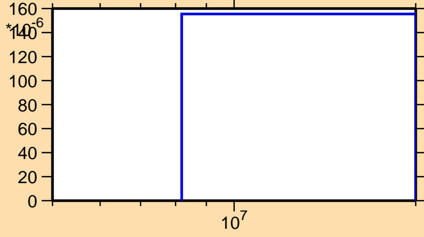
\sigma vs. E for ^{149}\text{La}(n,p)
