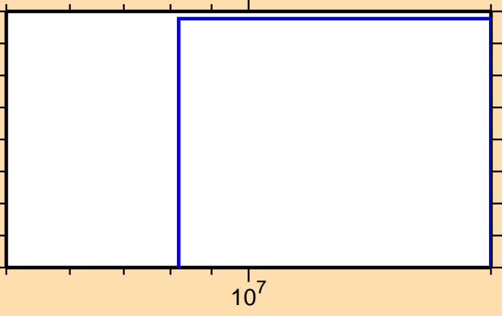
\sigma vs. E for ^{149}\text{La}(n,p)
