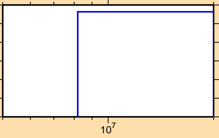
\sigma vs. E for ^{149}\text{La}(n,t)
