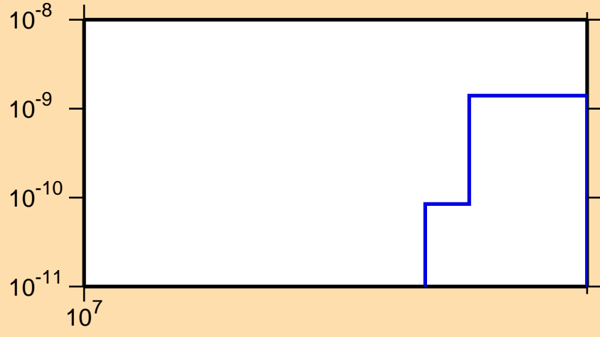
\sigma vs. E for ^{253}\text{Lw} (mt 34)
