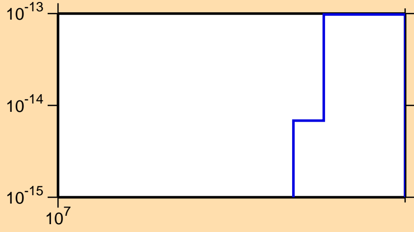
\sigma vs. E for ^{253}\text{Lw}(n,\text{pd})
