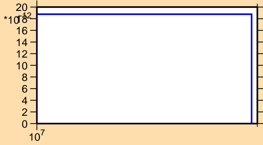
\sigma vs. E for ^{253}\text{Lw} (mt 34)
