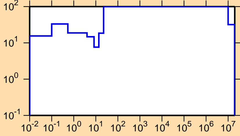
\Delta\sigma/\sigma vs. E for ^{253}\text{Lw}(n,f)
