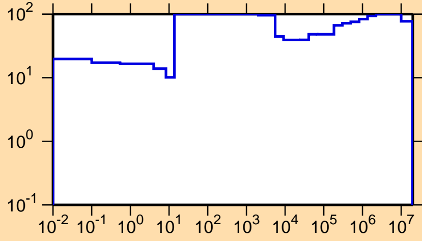
\Delta\sigma/\sigma vs. E for ^{253}\text{Lw}(n,\gamma)
