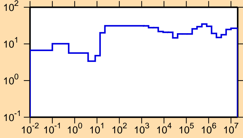
\Delta\sigma/\sigma vs. E for ^{253}\text{Lw}(n,el.)
