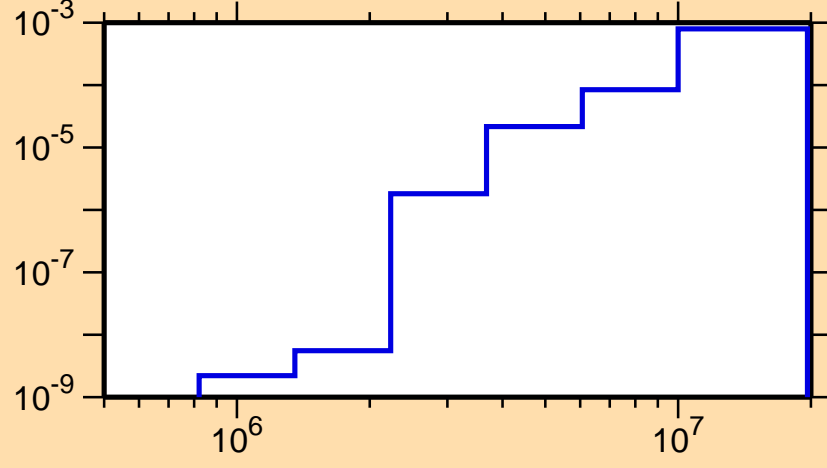
\sigma vs. E for ^{253}\text{Lw}(n,n\alpha)
