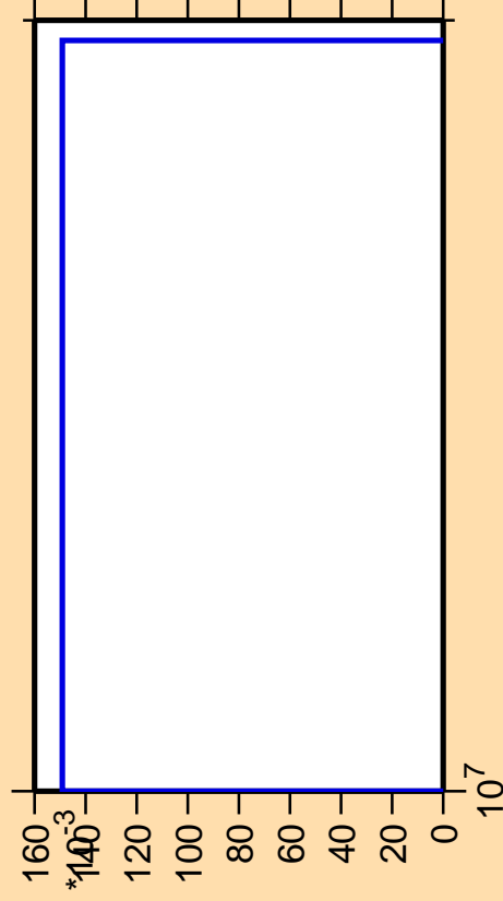
\Delta\sigma/\sigma vs. E for ^{253}\text{Lw}(n,pt)
