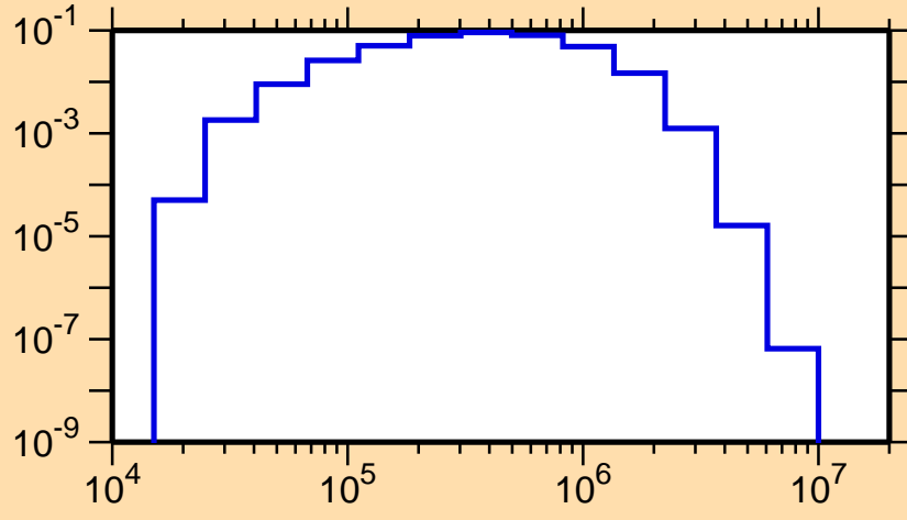
\sigma vs. E for ^{253}\text{Lw}(n,n_4)
