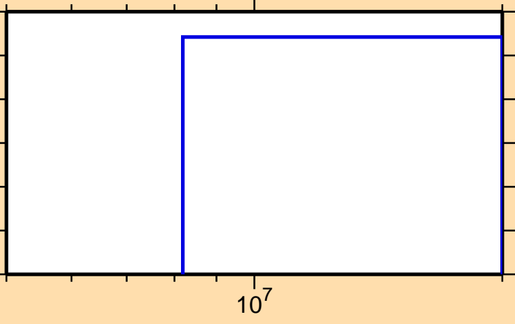
\sigma vs. E for ^{253}\text{Lw}(n,pt)
