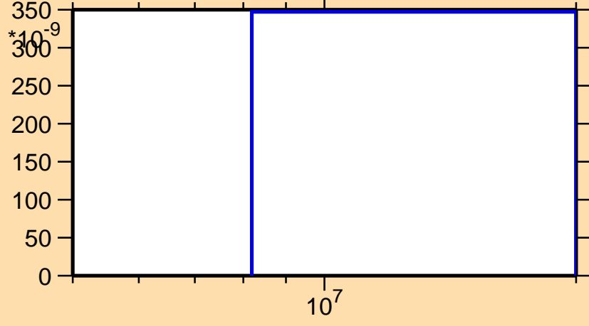
\sigma vs. E for ^{253}\text{Lw}(n,3n\alpha)
