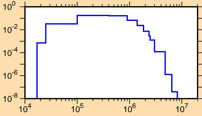
\sigma vs. E for ^{253}\text{Lw}(n,n_3)
