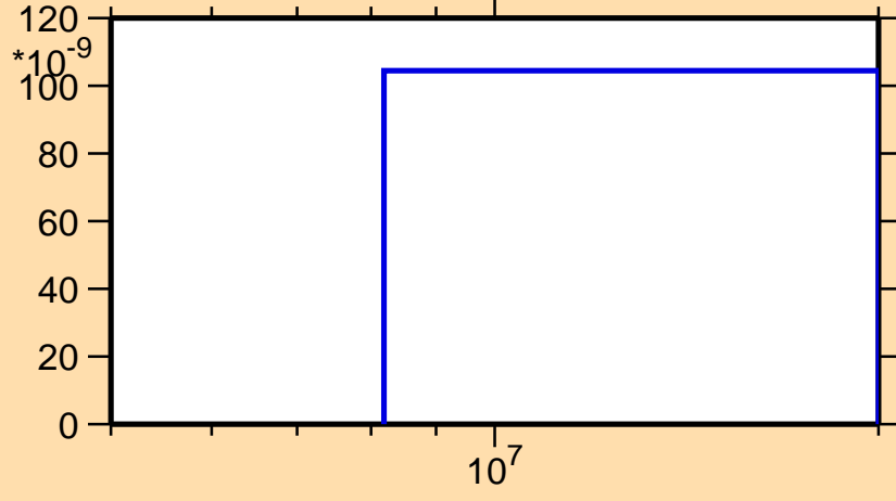
\sigma vs. E for ^{253}\text{Lw}(n,\text{He3})
