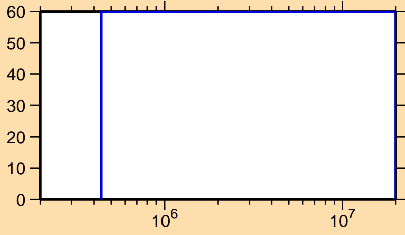
\Delta\sigma/\sigma vs. E for ^{254}\text{Lw}(n,n\text{cont.})
