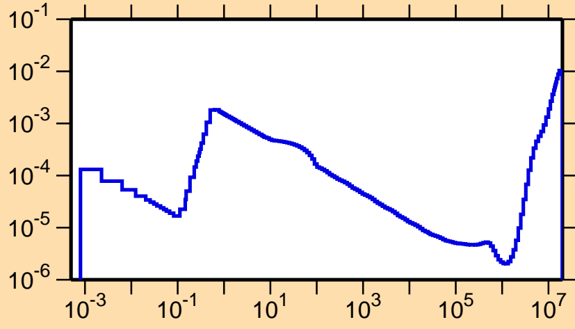
\sigma vs. E for ^{254}\text{Lw}(n,p)
