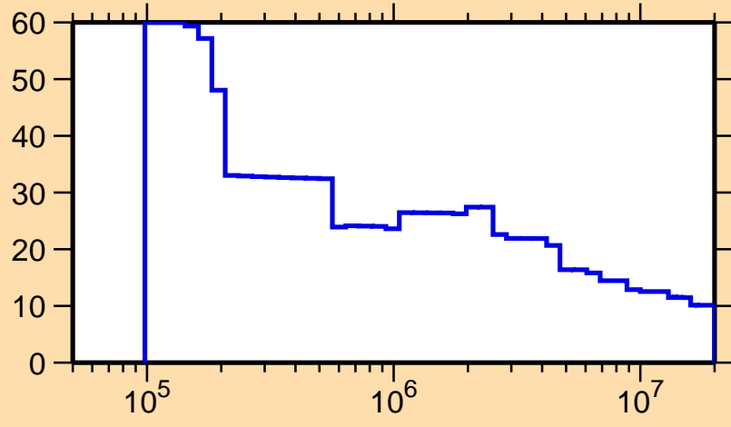
\Delta\sigma/\sigma vs. E for ^{254}\text{Lw}(n,\text{nonel.})
