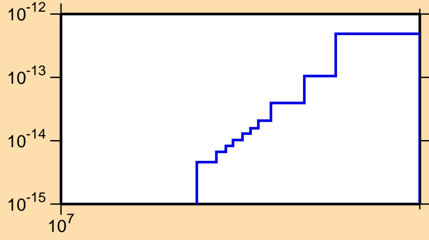
\sigma vs. E for ^{254}\text{Lw}(\text{mt117})
