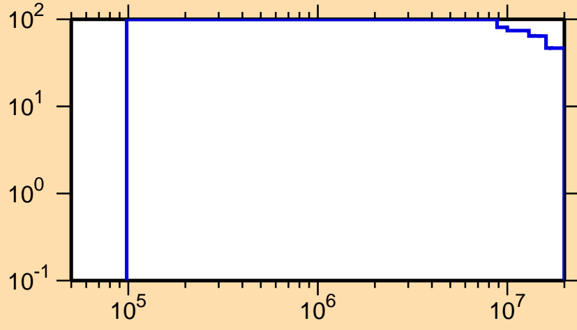
\Delta\sigma/\sigma vs. E for ^{254}\text{Lw}(n,f)
