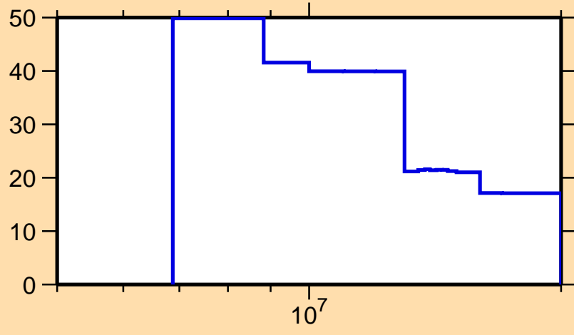
\Delta\sigma/\sigma vs. E for ^{254}\text{Lw}(n,\text{el.})
