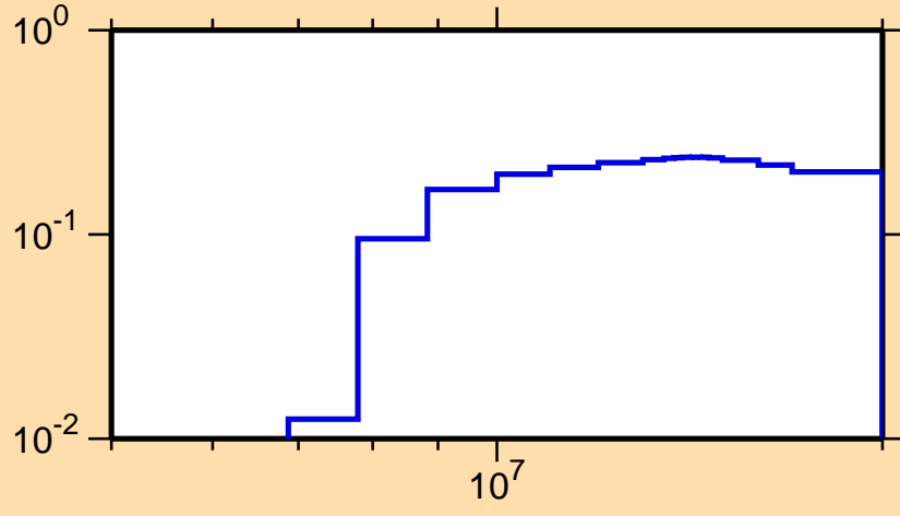
\sigma vs. E for ^{254}\text{Lw}(n,2n)
