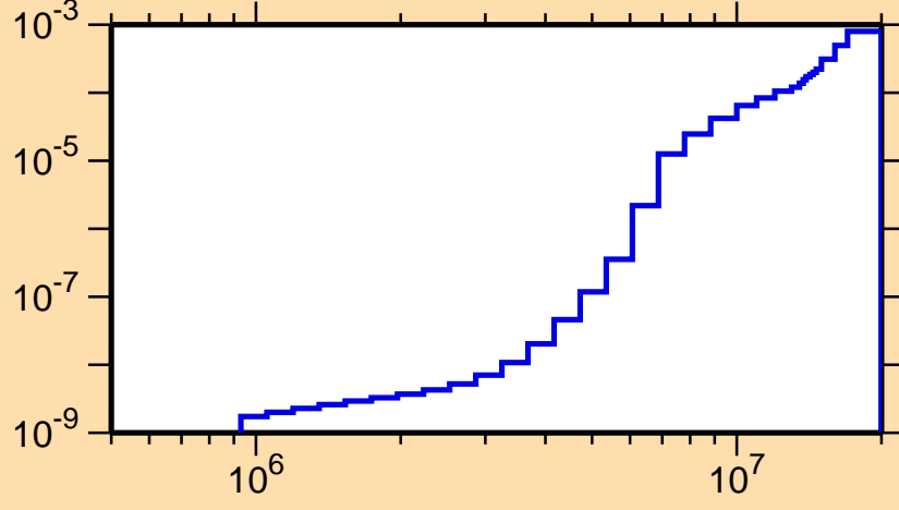
\sigma vs. E for ^{254}\text{Lw}(n,n\alpha)
