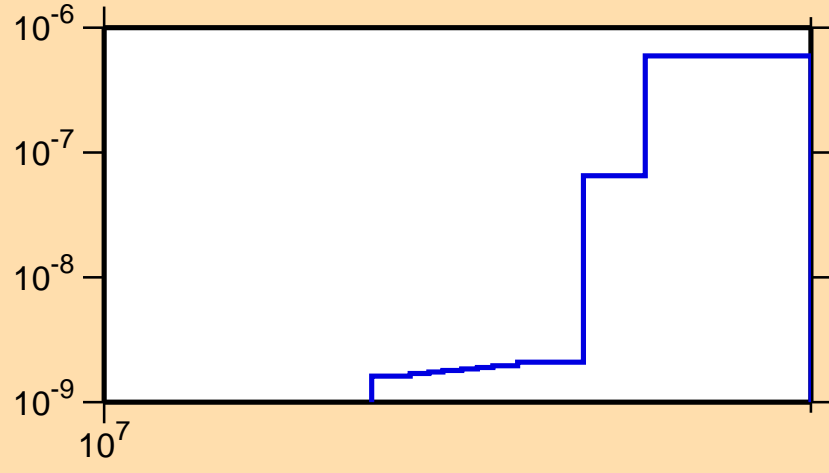
\sigma vs. E for ^{254}\text{Lw}(n,3n\alpha)
