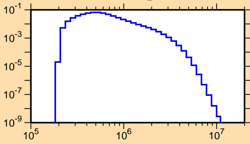
\sigma vs. E for ^{254}\text{Lw}(n,n_2)
