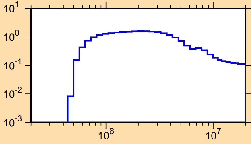
\sigma vs. E for ^{254}\text{Lw}(n,n\text{cont.})
