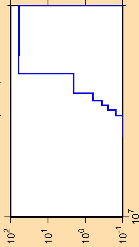
\Delta\sigma/\sigma vs. E for ^{254}\text{Lw}(\text{mt } 45)
