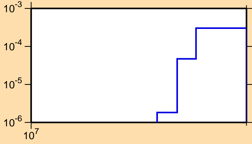
\sigma vs. E for ^{254}\text{Lw}(n,3n)
