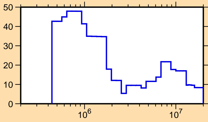
\Delta\sigma/\sigma vs. E for ^{254}\text{Lw}(n,\text{tot.})
