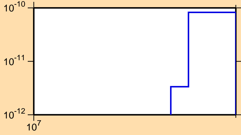
\sigma vs. E for ^{254}\text{Lw}(\text{mt 34})
