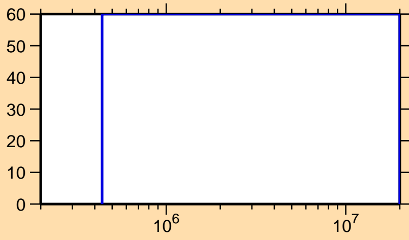
\Delta\sigma/\sigma vs. E for ^{254}\text{Lw}(n,n\text{cont.})
