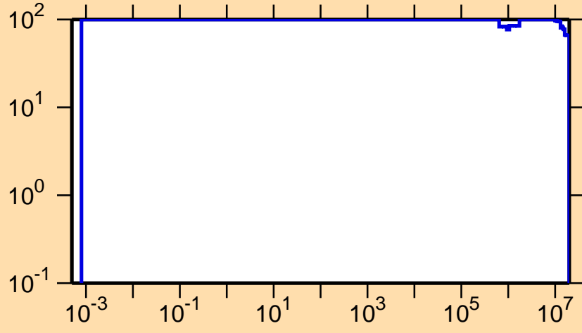
\Delta\sigma/\sigma vs. E for ^{254}\text{Lw}(n,p)
