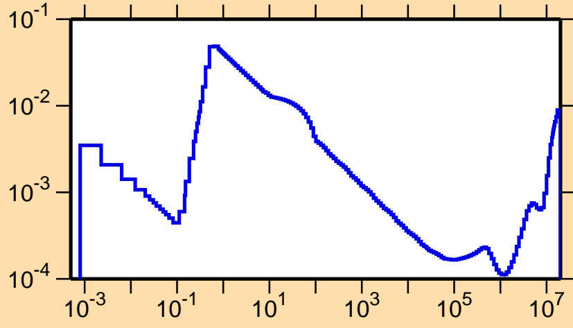
\sigma vs. E for ^{254}\text{Lw}(n,\alpha)
