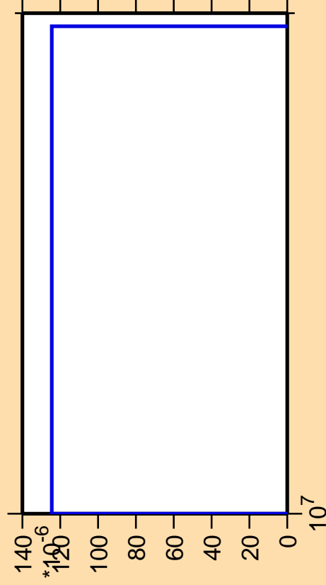
\Delta\sigma/\sigma vs. E for ^{254}\text{Lw}(n,pt)
