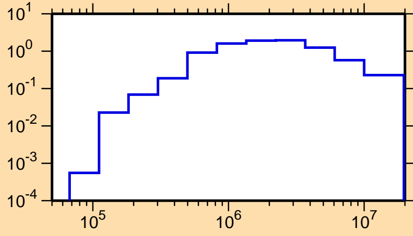
\sigma vs. E for ^{254}\text{Lw}(n,\text{inel.})
