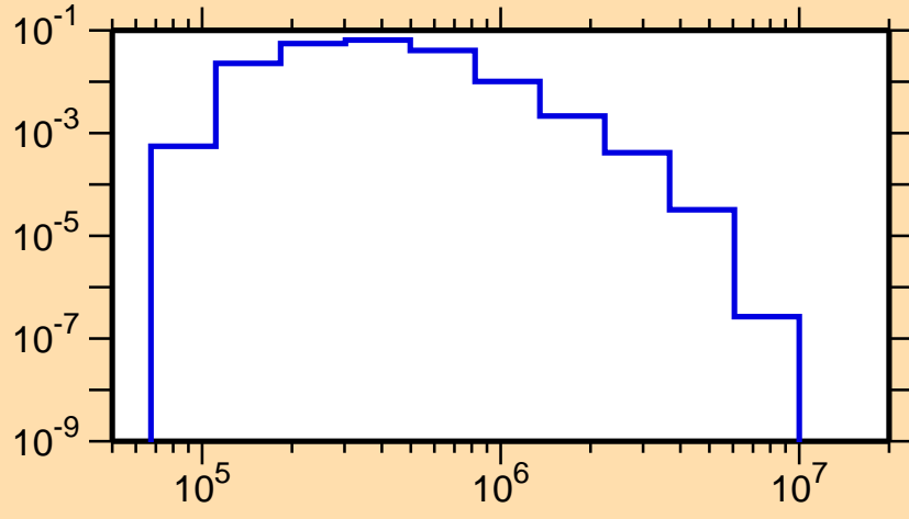
\sigma vs. E for ^{254}\text{Lw}(n,n_1)
