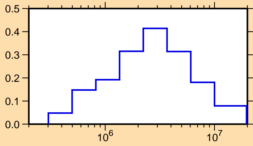
\sigma vs. E for ^{254}\text{Lw}(n,n_4)
