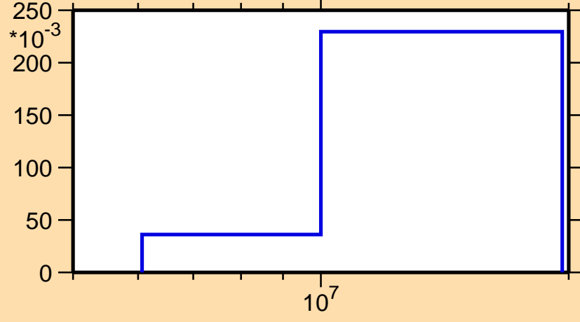
\sigma vs. E for ^{254}\text{Lw}(n,2n)
