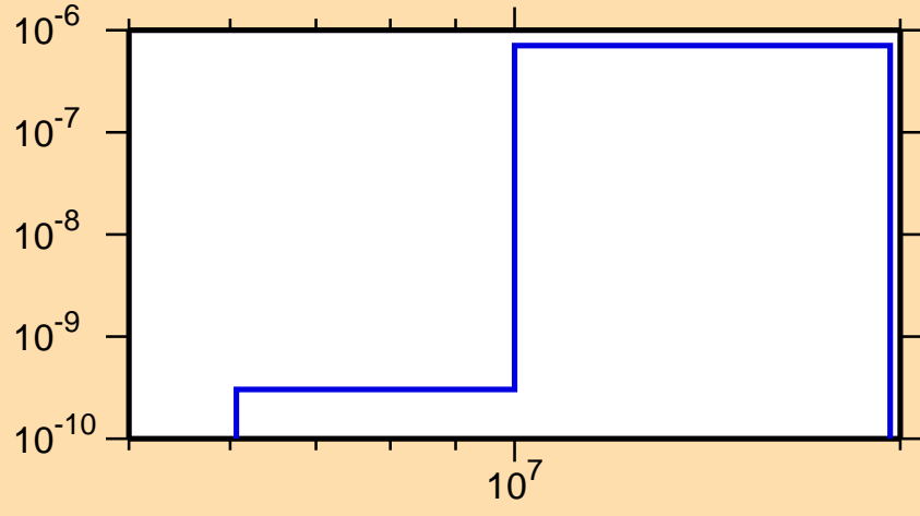
\sigma vs. E for ^{254}\text{Lw}(n,2n\alpha)
