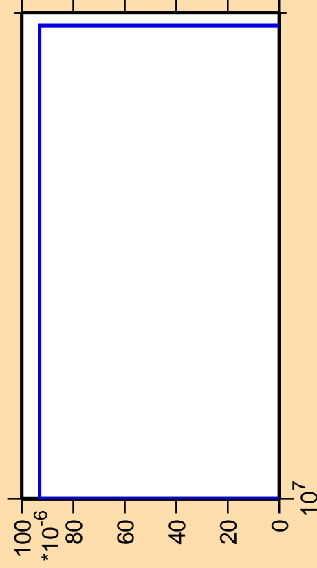
\Delta\sigma/\sigma vs. E for ^{254}\text{Lw}(n,\text{pd})
