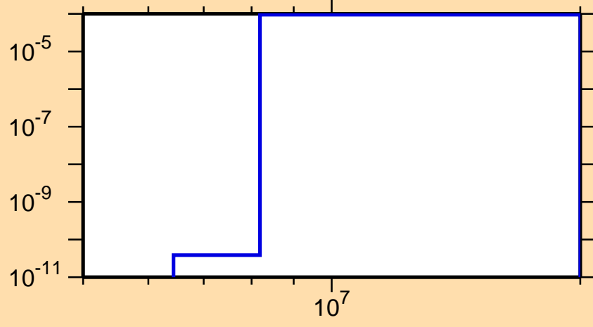
\sigma vs. E for ^{254}\text{Lw}(n,t)
