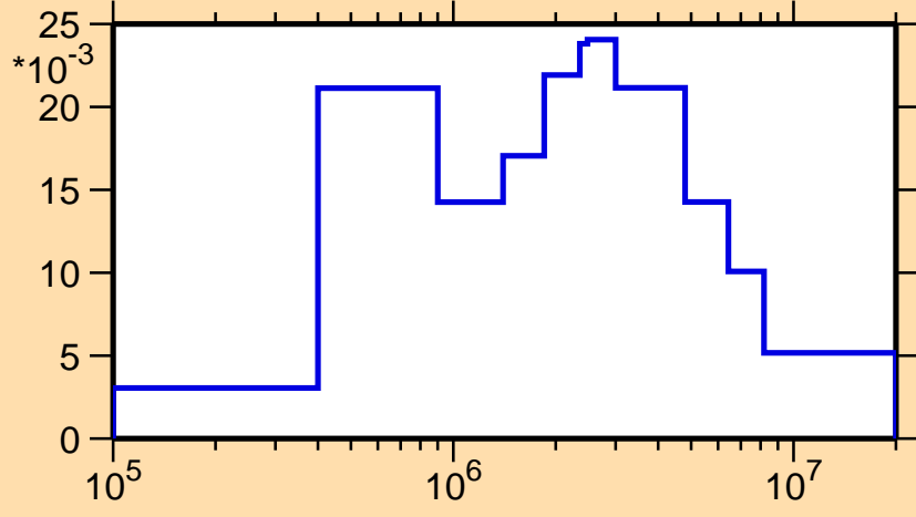
\sigma vs. E for ^{254}\text{Lw}(n,n_3)
