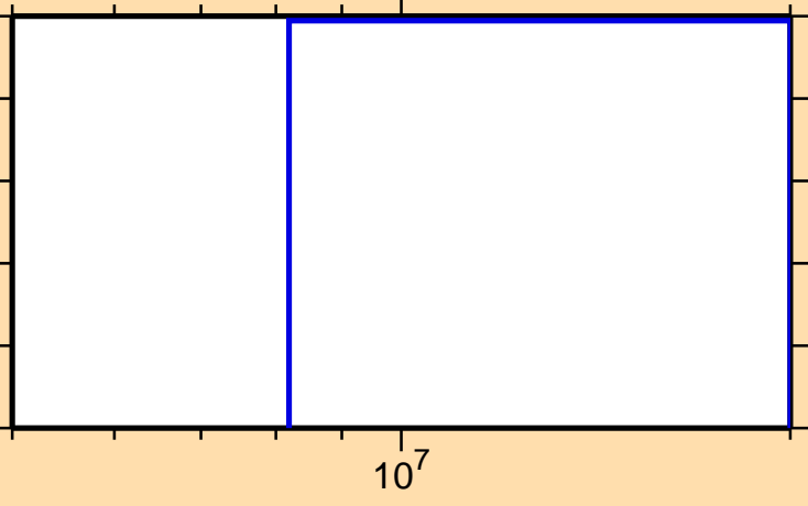
\sigma vs. E for ^{255}\text{Lw}(n,3n)
