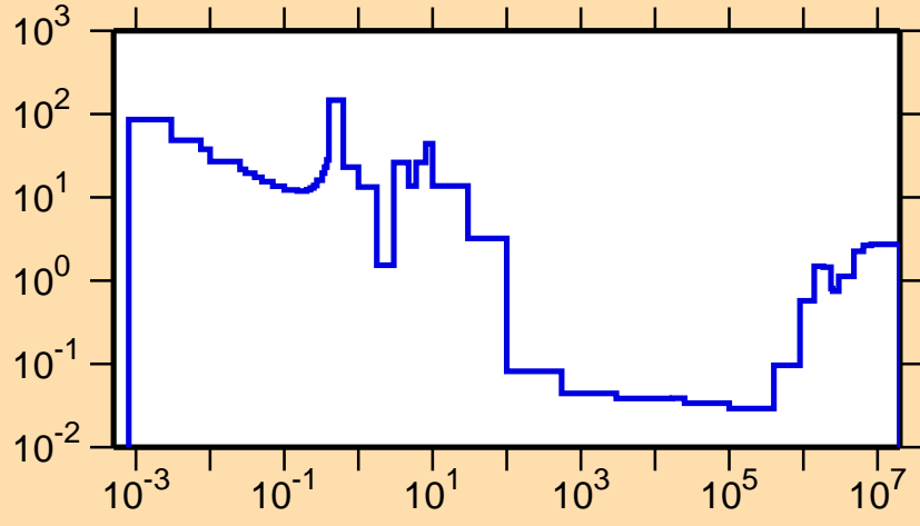
\sigma vs. E for ^{255}\text{Lw}(n,f)
