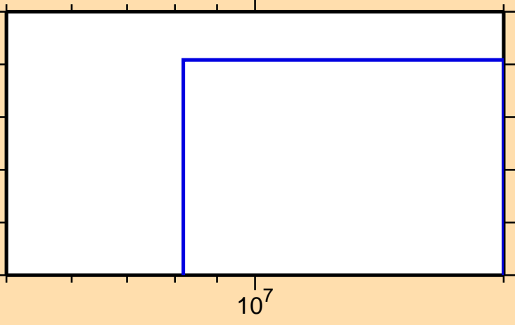
\sigma vs. E for ^{255}\text{Lw}(\text{mt117})
