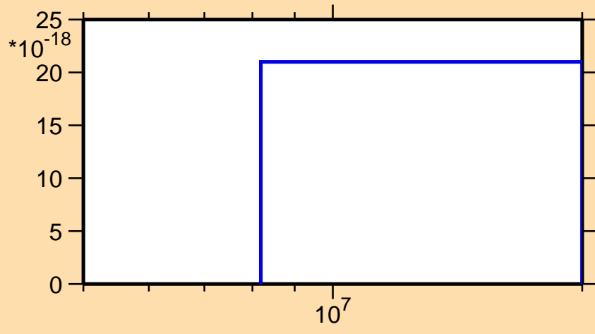
\sigma vs. E for ^{255}\text{Lw}(\text{mt } 34)
