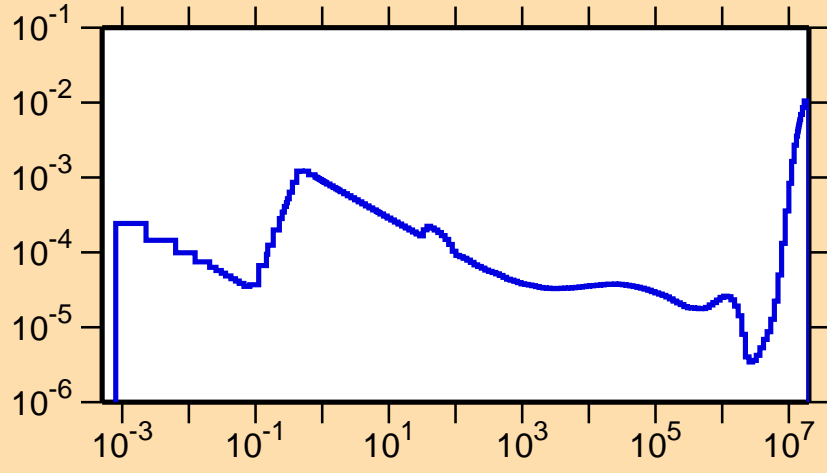
\sigma vs. E for ^{255}\text{Lw}(n,\alpha)
