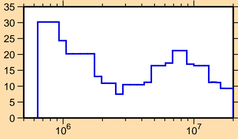
\Delta\sigma/\sigma vs. E for ^{255}\text{Lw}(n,\text{tot.})
