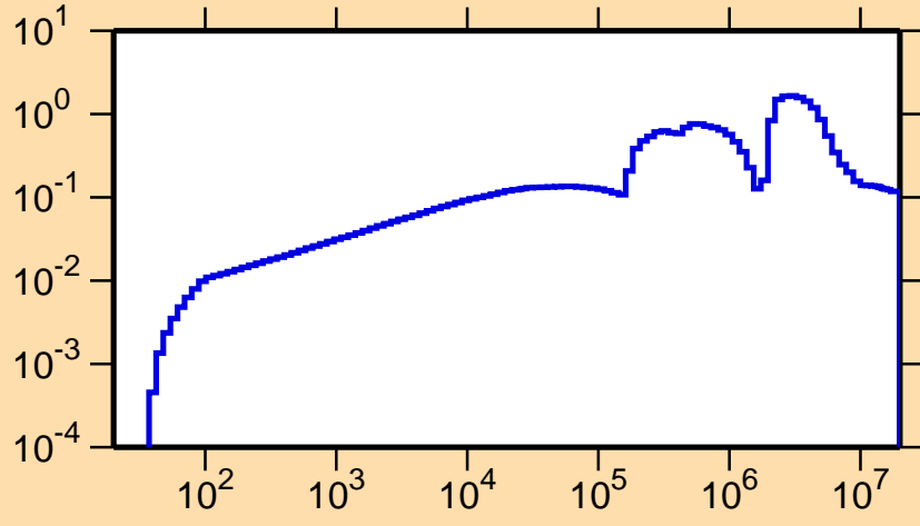
\sigma vs. E for ^{255}\text{Lw}(n,\text{inel.})
