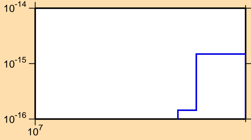
\sigma vs. E for ^{255}\text{Lw} (mt 34)
