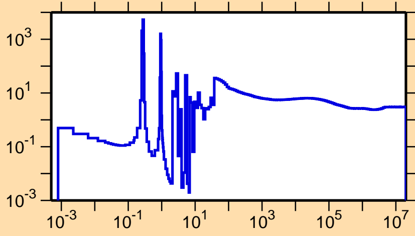
\sigma vs. E for ^{255}\text{Lw}(n,\text{nonel.})
