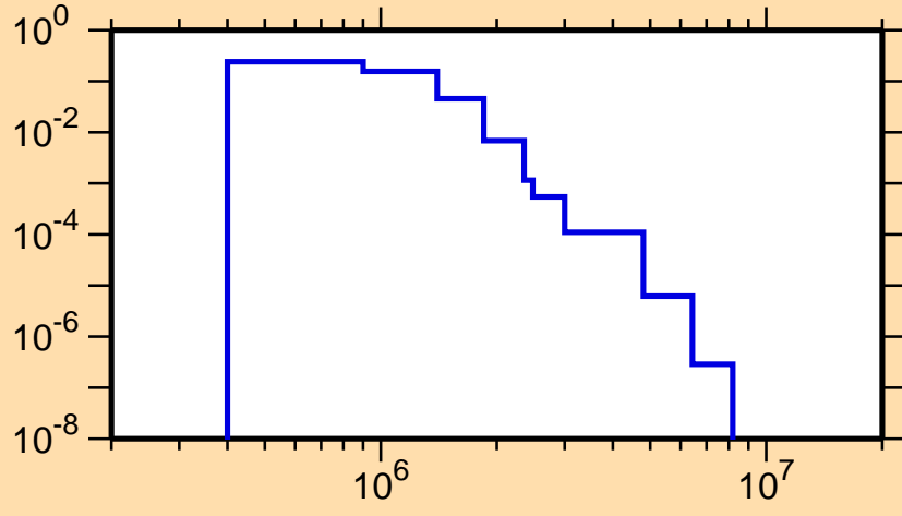
\sigma vs. E for ^{255}\text{Lw}(n,n_3)
