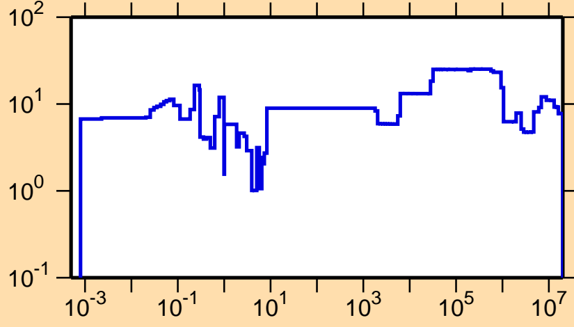
\Delta\sigma/\sigma vs. E for ^{256}\text{Lw}(n,\text{tot.})
