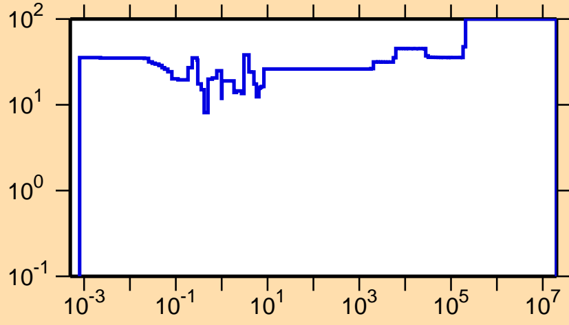
\Delta\sigma/\sigma vs. E for ^{256}\text{Lw}(n,\gamma)
