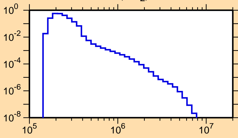
\sigma vs. E for ^{256}\text{Lw}(n, n_2)
