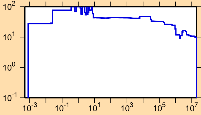
\Delta\sigma/\sigma vs. E for ^{256}\text{Lw}(n,\text{nonel.})
