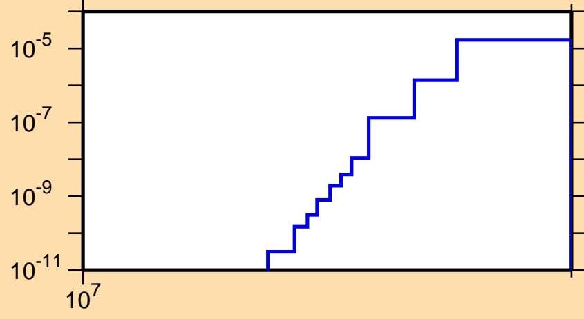
\sigma vs. E for ^{256}\text{Lw}(n,nt)
