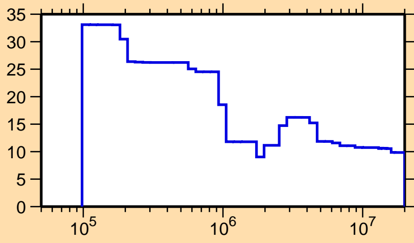
\Delta\sigma/\sigma vs. E for ^{256}\text{Lw}(n,\text{nonel.})
