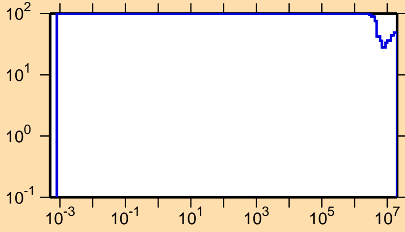
\Delta\sigma/\sigma vs. E for ^{256}\text{Lw}(n,p)
