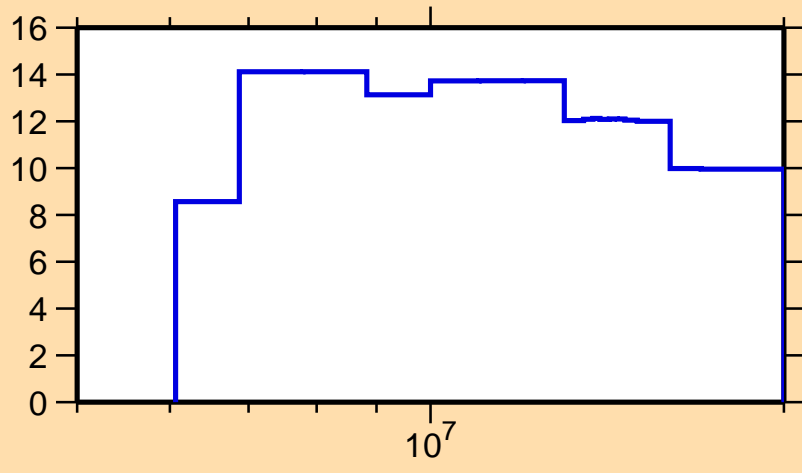
\Delta\sigma/\sigma vs. E for ^{256}\text{Lw}(n,\text{el.})
