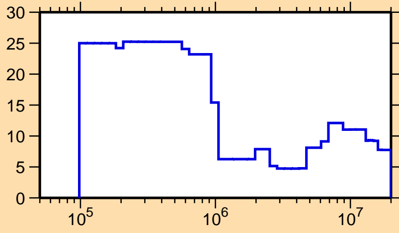
\Delta\sigma/\sigma vs. E for ^{256}\text{Lw}(n,\text{tot.})
