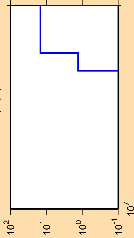
\Delta\sigma/\sigma vs. E for ^{256}\text{Lw}(n,\text{pt})
