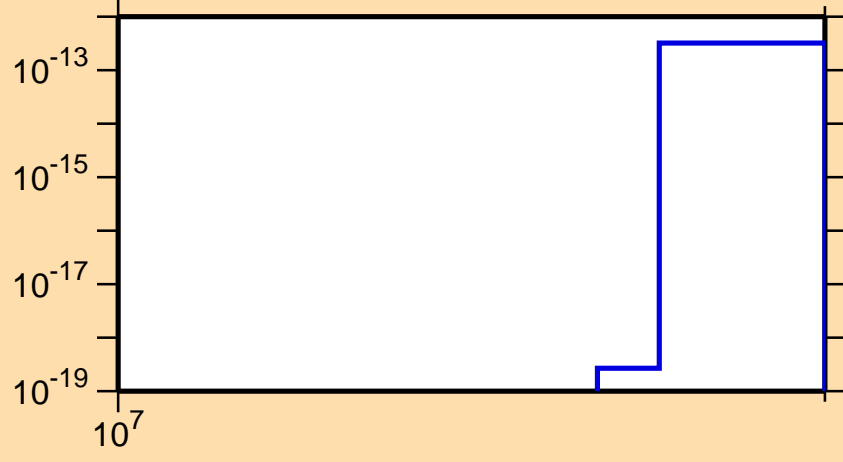
\sigma vs. E for ^{256}\text{Lw} (mt 11)
