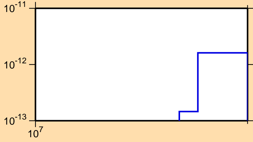
\sigma vs. E for ^{256}\text{Lw}(n,\text{pt})
