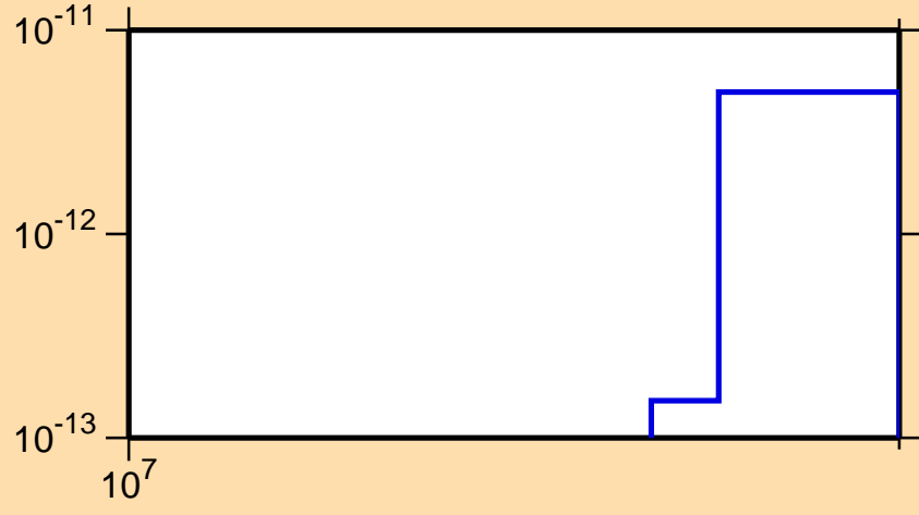
\sigma vs. E for ^{256}\text{Lw}(n,\text{pd})
