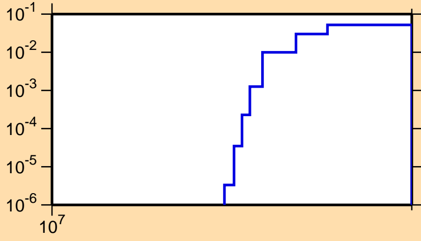
\sigma vs. E for ^{256}\text{Lw}(n,3n)
