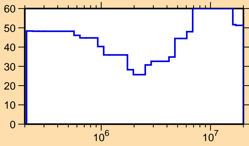
\Delta\sigma/\sigma vs. E for ^{256}\text{Lw}(n,\text{inel.})
