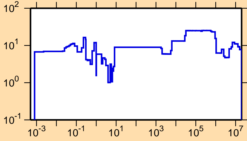
\Delta\sigma/\sigma vs. E for ^{256}\text{Lw}(n,tot.)
