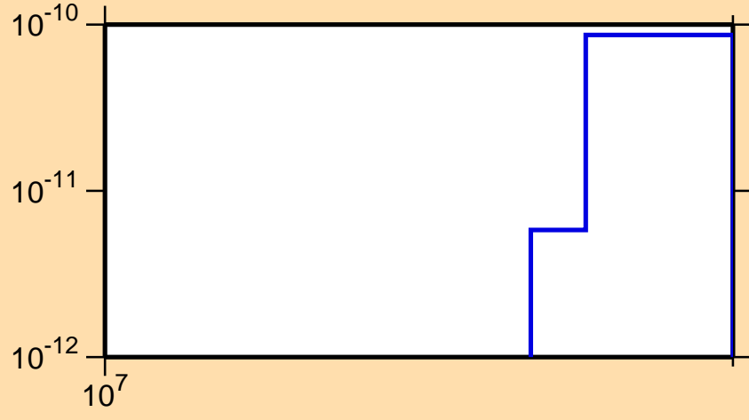
\sigma vs. E for ^{256}\text{Lw} (mt 34)
