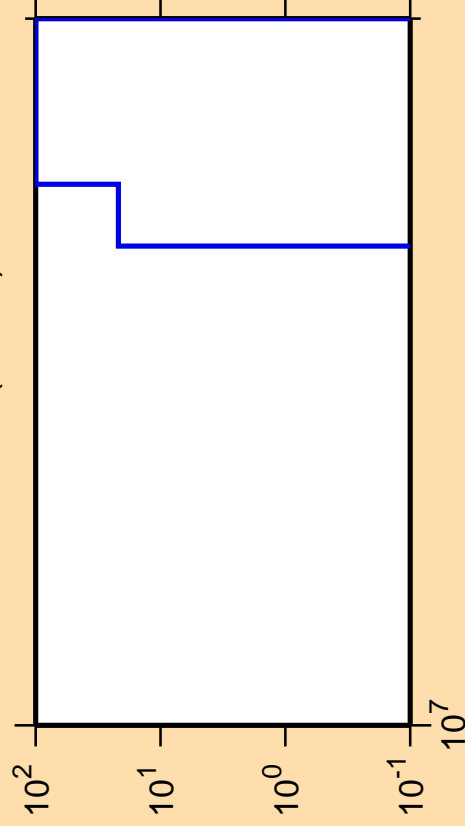
\Delta\sigma/\sigma vs. E for ^{256}\text{Lw} (mt 34)
