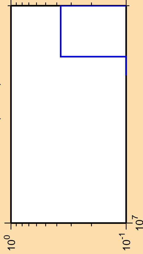
\Delta\sigma/\sigma vs. E for ^{256}\text{Lw} (mt 11)
