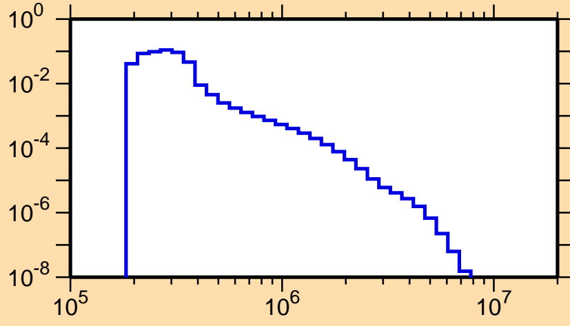
\sigma vs. E for ^{256}\text{Lw}(n,n_3)
