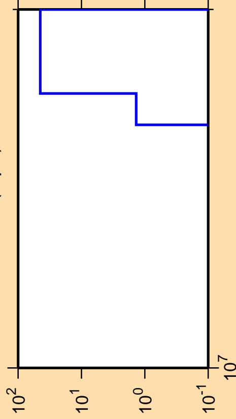
\Delta\sigma/\sigma vs. E for ^{256}\text{Lw}(n,\text{pd})
