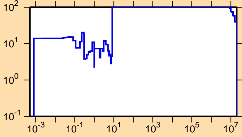
\Delta\sigma/\sigma vs. E for ^{256}\text{Lw}(n,f)
