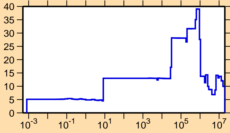
\Delta\sigma/\sigma vs. E for ^{256}\text{Lw}(n,\text{el.})
