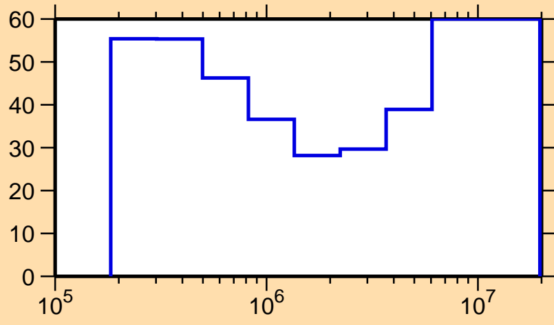
\Delta\sigma/\sigma vs. E for ^{256}\text{Lw}(n,ncont.)
