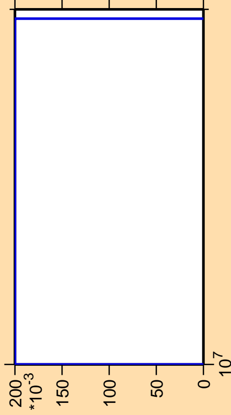
\Delta\sigma/\sigma vs. E for ^{256}\text{Lw}(n,pt)
