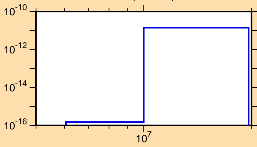
\sigma vs. E for ^{256}\text{Lw}(mt117)
