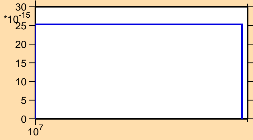
\sigma vs. E for ^{256}\text{Lw}(n,pt)
