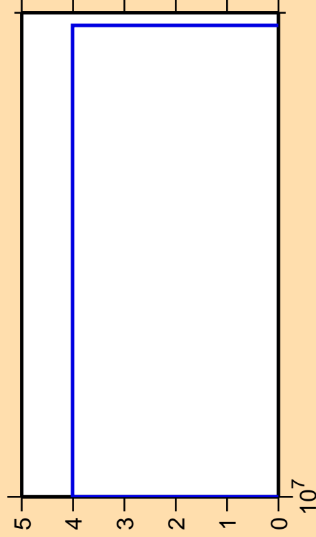
\Delta\sigma/\sigma vs. E for ^{256}\text{Lw} (mt 34)
