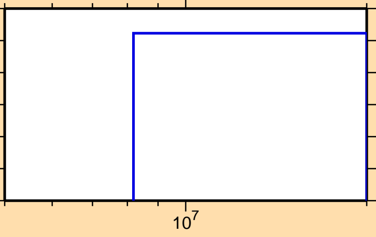
\sigma vs. E for ^{256}\text{Lw}(\text{mt } 11)
