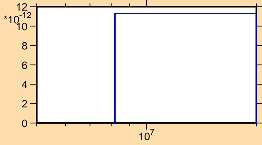
\sigma vs. E for ^{256}\text{Lw}(\text{mt117})
