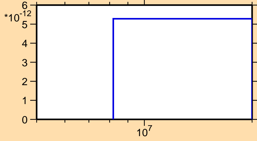
\sigma vs. E for ^{256}\text{Lw} (mt 45)
