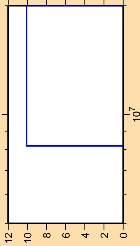
\Delta\sigma/\sigma vs. E for ^{256}\text{Lw} (mt 45)
