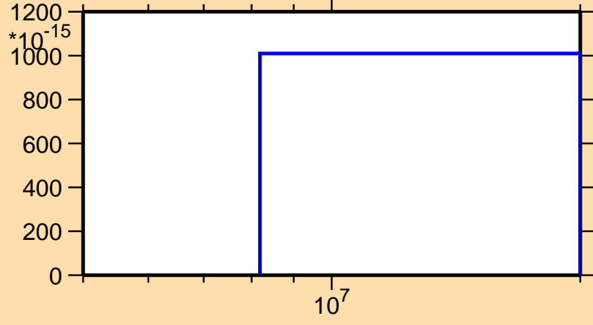
\sigma vs. E for ^{256}\text{Lw}(\text{mt } 34)
