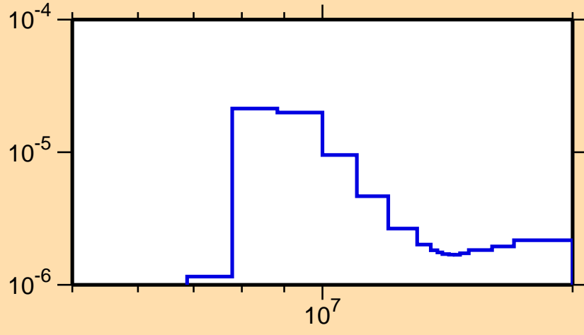
\sigma vs. E for ^{257}\text{Lw}(n,2n\alpha)
