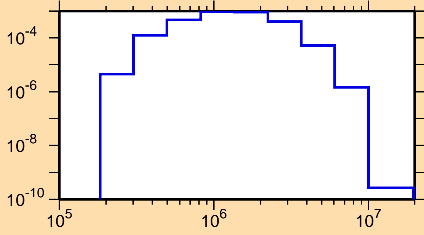
\sigma vs. E for ^{257}\text{Lw}(n,n_3)
