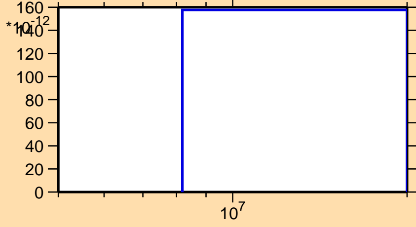
\sigma vs. E for ^{257}\text{Lw}(n,\text{He3})
