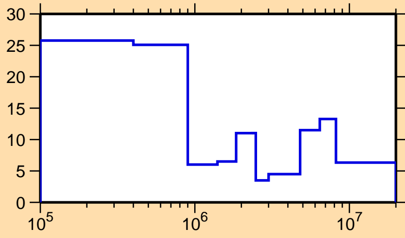
\Delta\sigma/\sigma vs. E for ^{257}\text{Lw}(n,\text{tot.})
