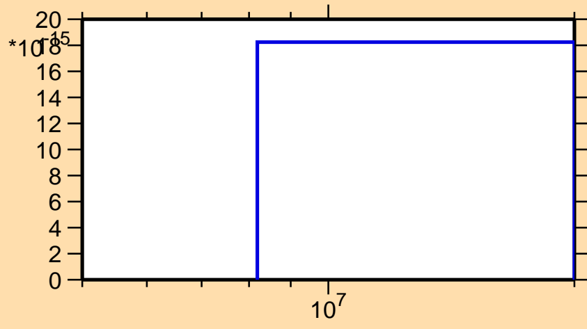
\sigma vs. E for ^{257}\text{Lw}(\text{mt 11})
