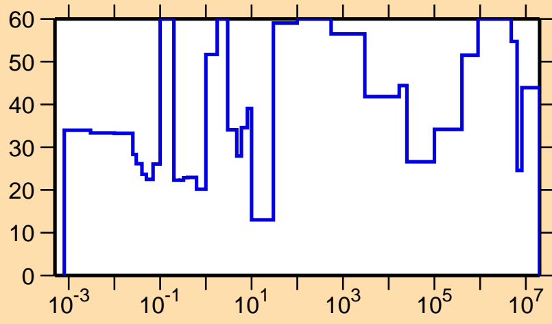
\Delta\sigma/\sigma vs. E for ^{257}\text{Lw}(n,\gamma)
