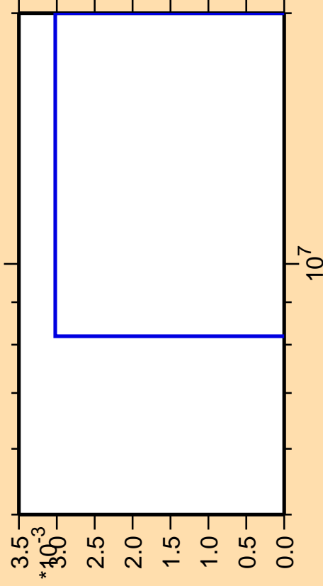
\Delta\sigma/\sigma vs. E for ^{257}\text{Lw} (mt 42)
