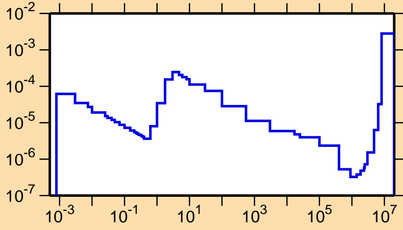
\sigma vs. E for ^{257}\text{Lw}(n,\alpha)
