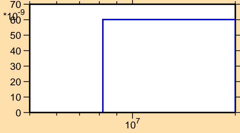
\sigma vs. E for ^{257}\text{Lw}(n,nt)
