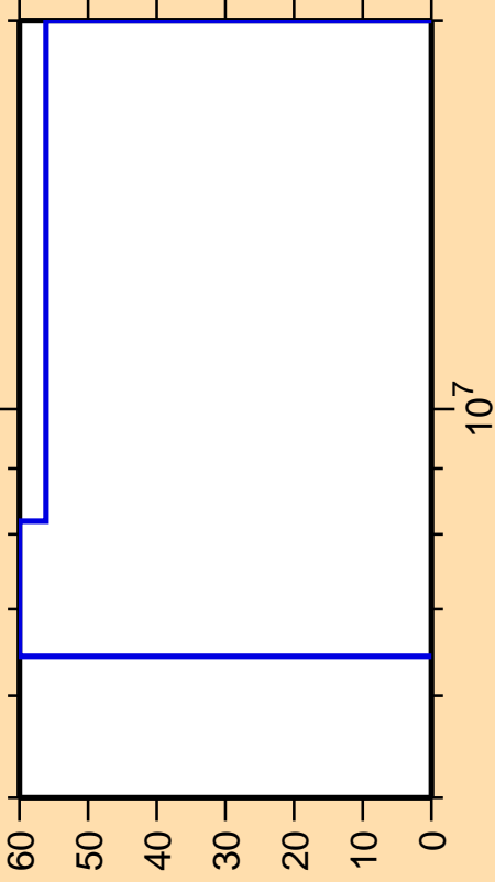
\Delta\sigma/\sigma vs. E for ^{257}\text{Lw}(n, n_{\text{cont}})
