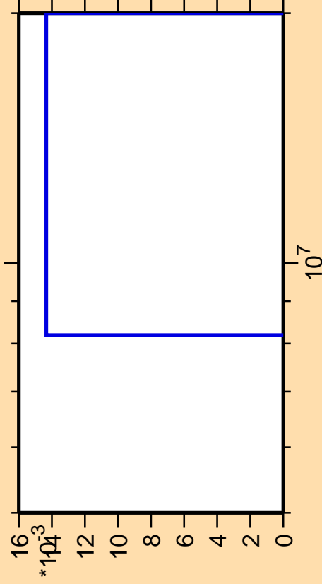
\Delta\sigma/\sigma vs. E for ^{257}\text{Lw}(\text{mt 11})
