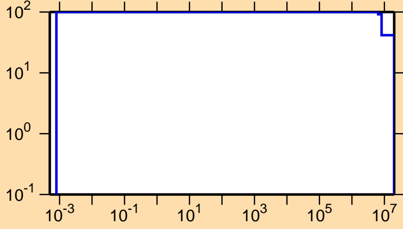
\Delta\sigma/\sigma vs. E for ^{257}\text{Lw}(n,p)
