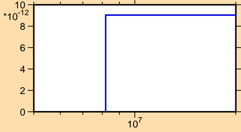
\sigma vs. E for ^{257}\text{Lw} (mt 45)
