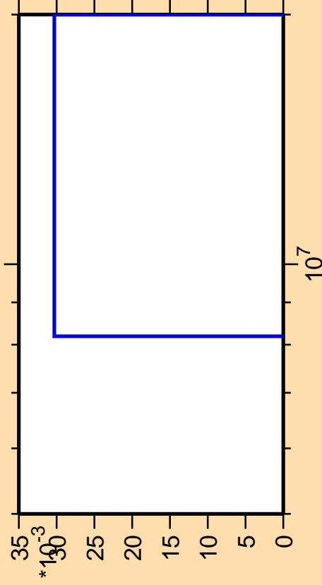
\Delta\sigma/\sigma vs. E for ^{257}\text{Lw}(\text{mt } 34)
