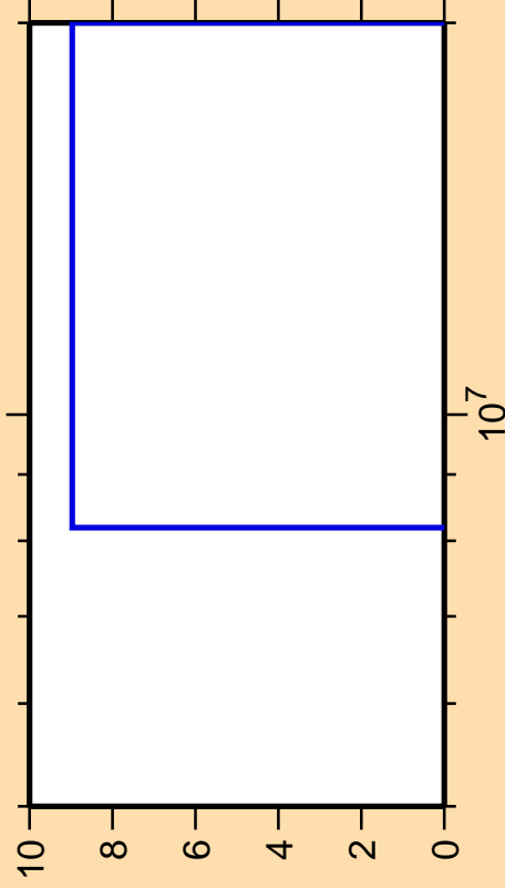
\Delta\sigma/\sigma vs. E for ^{257}\text{Lw} (mt 45)
