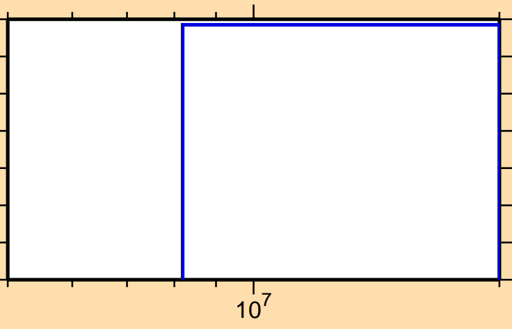
\sigma vs. E for ^{257}\text{Lw}(n,3n)
