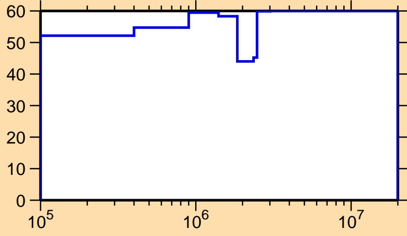
\Delta\sigma/\sigma vs. E for ^{257}\text{Lw}(n,n_1)
