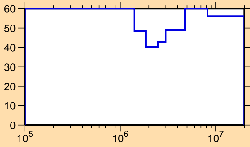
\Delta\sigma/\sigma vs. E for ^{257}\text{Lw}(n,n\text{cont.})
