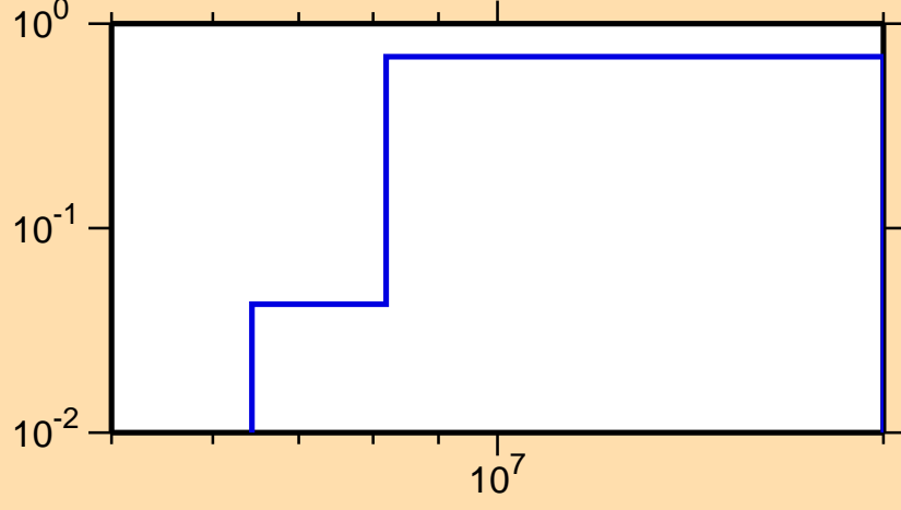
\sigma vs. E for ^{257}\text{Lw}(n,2n)
