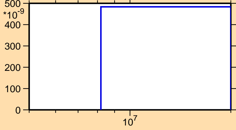
\sigma vs. E for ^{257}\text{Lw}(n,2np)
