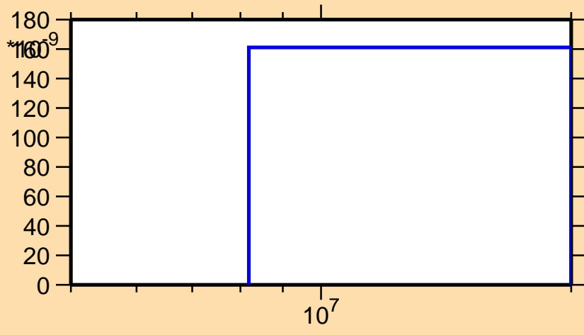
\sigma vs. E for ^{257}\text{Lw}(n,nd)
