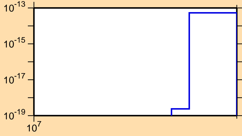
\sigma vs. E for ^{258}\text{Lw} (mt 11)
