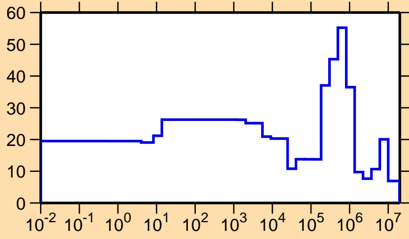
\Delta\sigma/\sigma vs. E for ^{258}\text{Lw}(n,el.)
