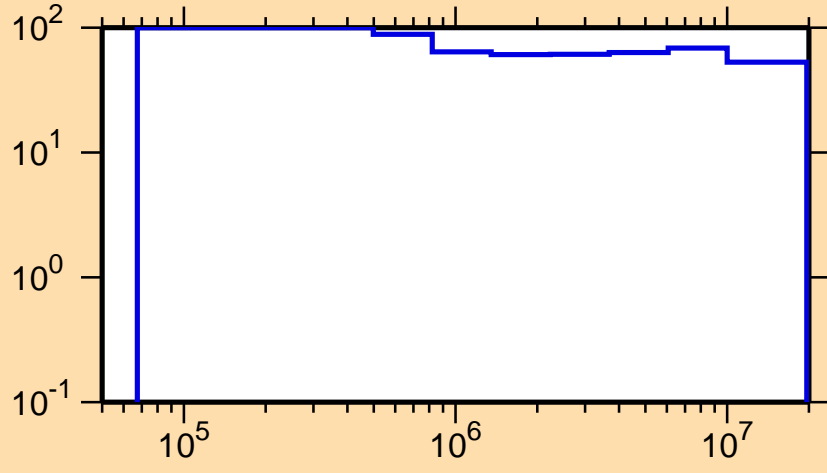
\Delta\sigma/\sigma vs. E for ^{258}\text{Lw}(n,n\text{cont.})
