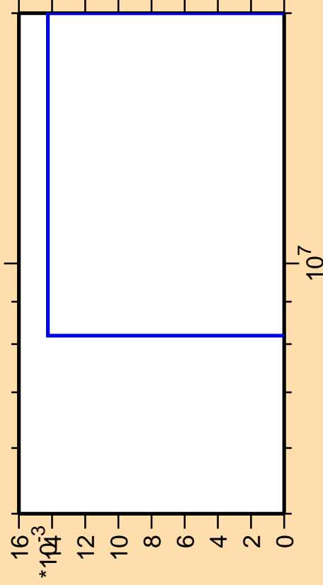
\Delta\sigma/\sigma vs. E for ^{258}\text{Lw}(\text{mt } 34)
