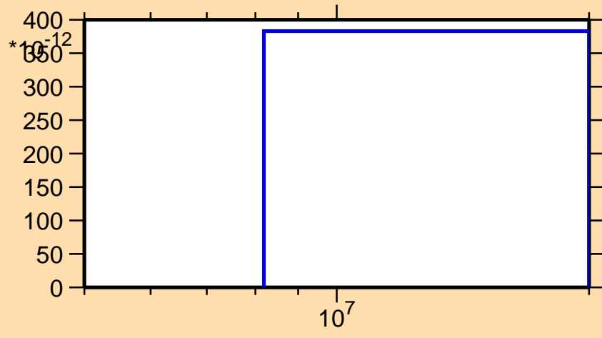
\sigma vs. E for ^{258}\text{Lw}(n,\text{He3})
