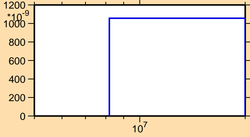
\sigma vs. E for ^{258}\text{Lw}(n,2np)
