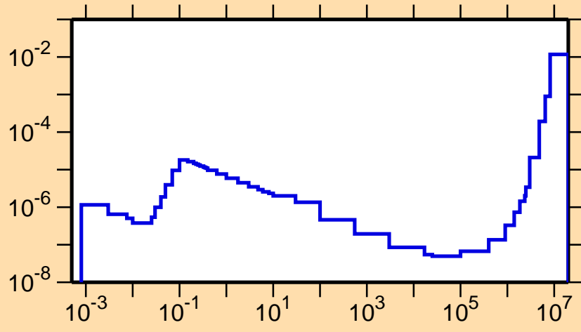
\sigma vs. E for ^{258}\text{Lw}(n,p)
