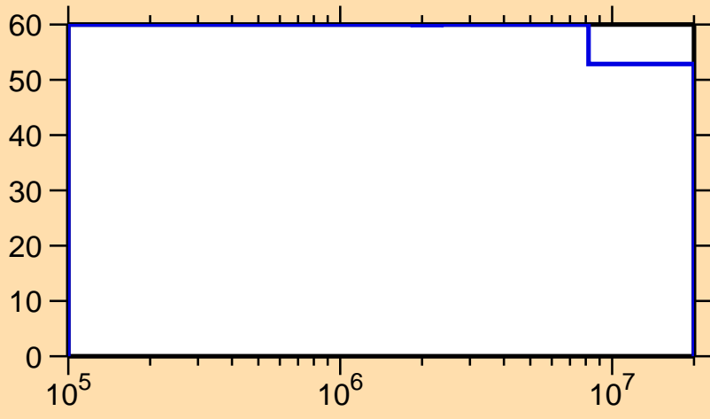
\Delta\sigma/\sigma vs. E for ^{258}\text{Lw}(n,\text{inel.})
