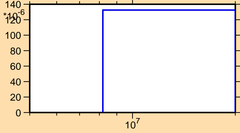
\sigma vs. E for ^{258}\text{Lw}(n,3n)
