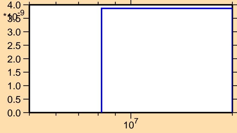
\sigma vs. E for ^{258}\text{Lw}(n,nt)
