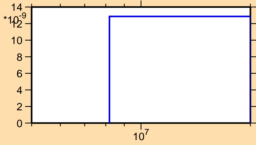
\sigma vs. E for ^{258}\text{Lw}(\text{mt117})
