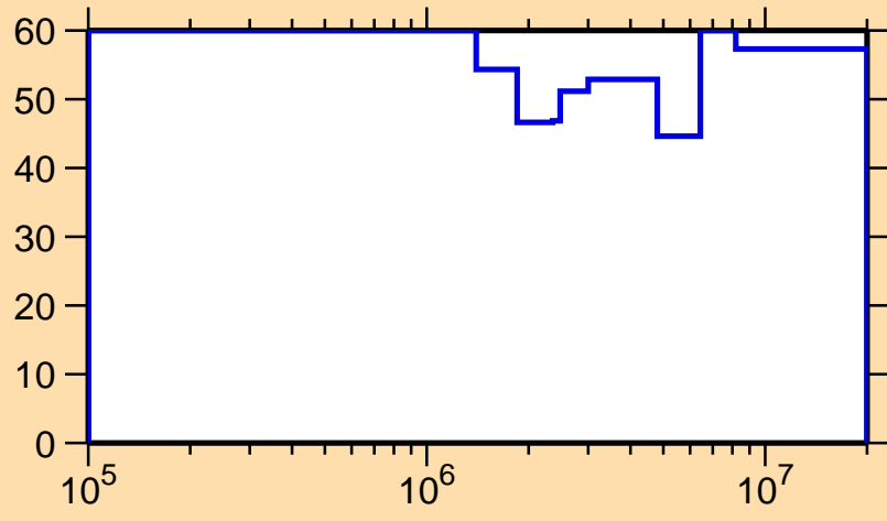
\Delta\sigma/\sigma vs. E for ^{258}\text{Lw}(n,n_1)
