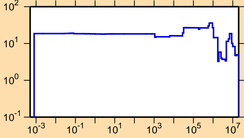
\Delta\sigma/\sigma vs. E for ^{259}\text{Lw}(n,el.)
