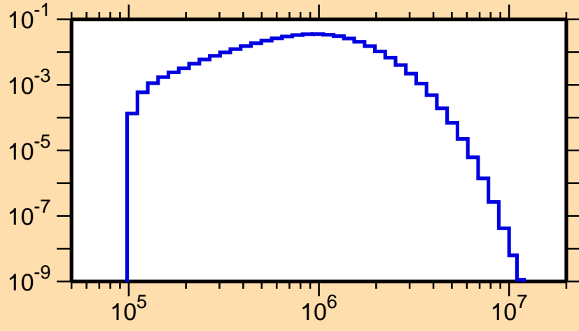
\sigma vs. E for ^{259}\text{Lw}(n,n_1)
