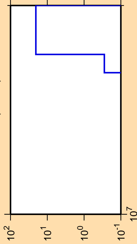
\Delta\sigma/\sigma vs. E for ^{259}\text{Lw} (mt 34)
