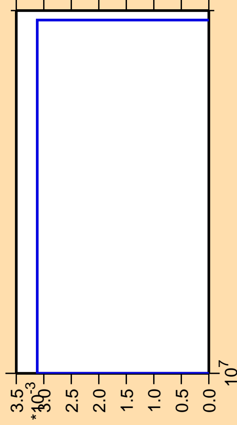
\Delta\sigma/\sigma vs. E for ^{259}\text{Lw}(\text{mt 11})
