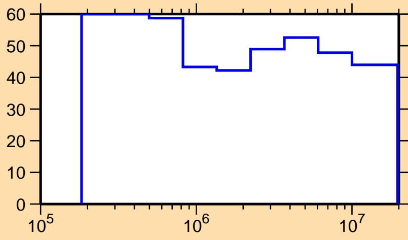
\Delta\sigma/\sigma vs. E for ^{259}\text{Lw}(n,ncont.)
