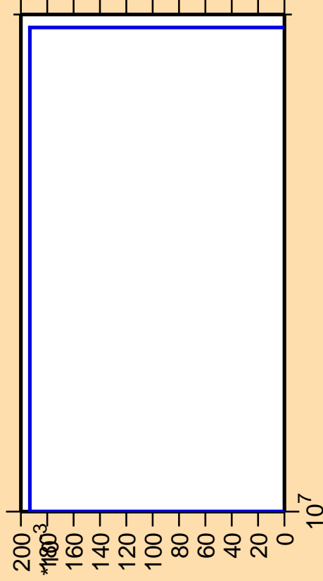
\Delta\sigma/\sigma vs. E for ^{259}\text{Lw} (mt 45)
