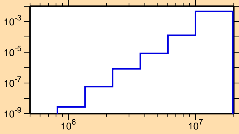
\sigma vs. E for ^{259}\text{Lw}(n,p)
