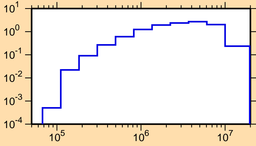
\sigma vs. E for ^{259}\text{Lw}(n,n\text{cont.})
