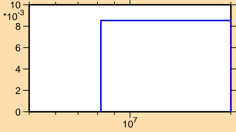
\sigma vs. E for ^{259}\text{Lw}(n,3n)
