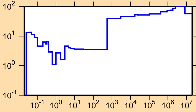
\Delta\sigma/\sigma vs. E for ^{259}\text{Lw}(n,\gamma)
