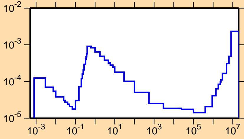
\sigma vs. E for ^{259}\text{Lw}(n,\alpha)
