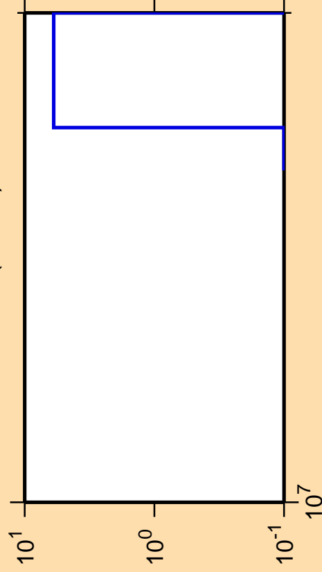
\Delta\sigma/\sigma vs. E for ^{261}\text{Lw} (mt 34)
