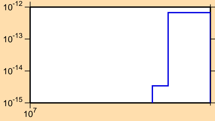
\sigma vs. E for ^{261}\text{Lw} (mt 34)
