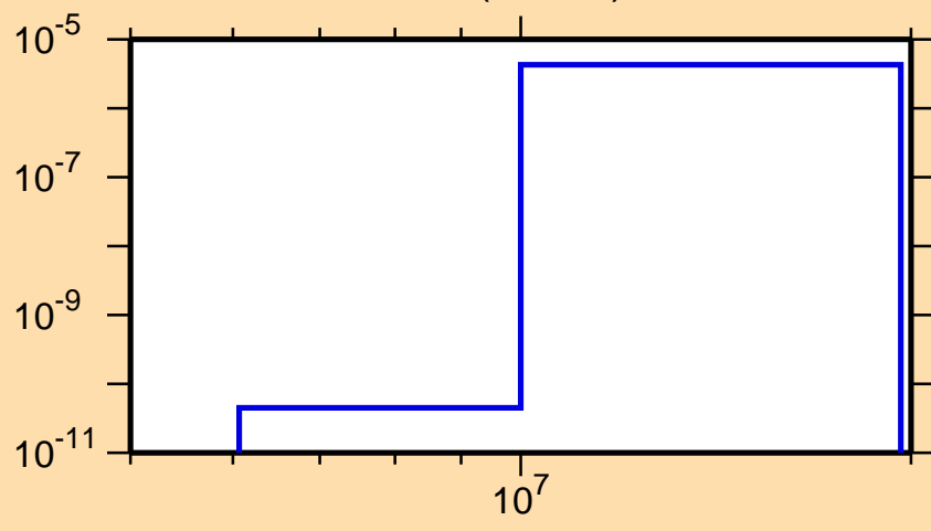
\sigma vs. E for ^{261}\text{Lw}(n,2n\alpha)
