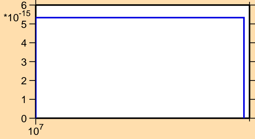
\sigma vs. E for ^{261}\text{Lw}(\text{mt } 34)
