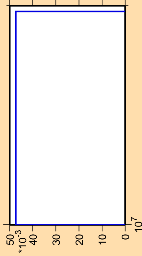
\Delta\sigma/\sigma vs. E for ^{261}\text{Lw}(\text{mt } 34)
