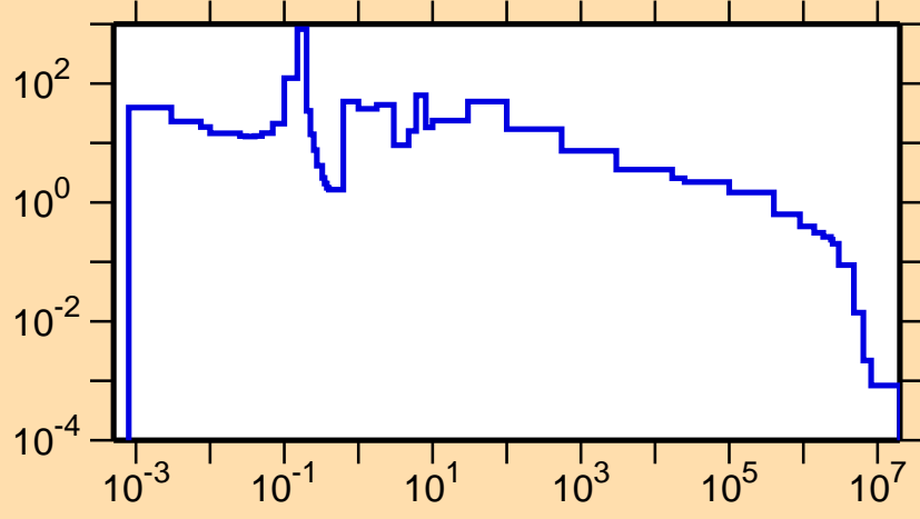
\sigma vs. E for ^{261}\text{Lw}(n,\gamma)
