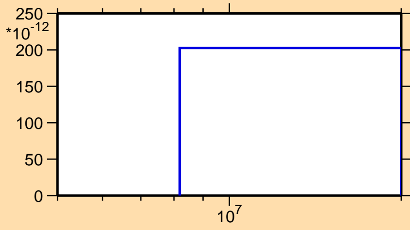
\sigma vs. E for ^{261}\text{Lw}(n,\text{He3})
