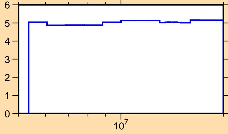
\Delta\sigma/\sigma vs. E for ^{262}\text{Lw}(n,\text{nonel.})
