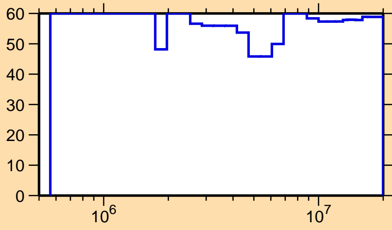
\Delta\sigma/\sigma vs. E for ^{262}\text{Lw}(n,n_1)
