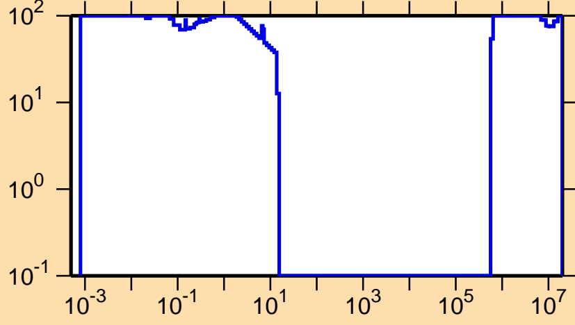
\Delta\sigma/\sigma vs. E for ^{262}\text{Lw}(n,p)
