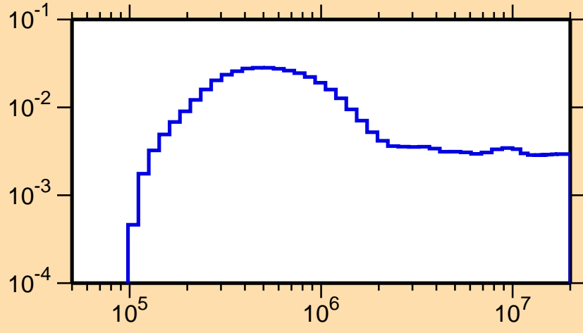
\sigma vs. E for ^{262}\text{Lw}(n,\text{inel.})
