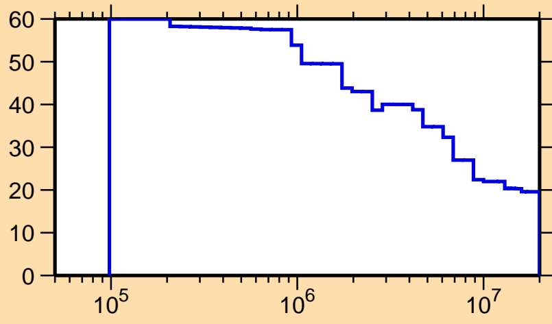
\Delta\sigma/\sigma vs. E for ^{262}\text{Lw}(n,f)
