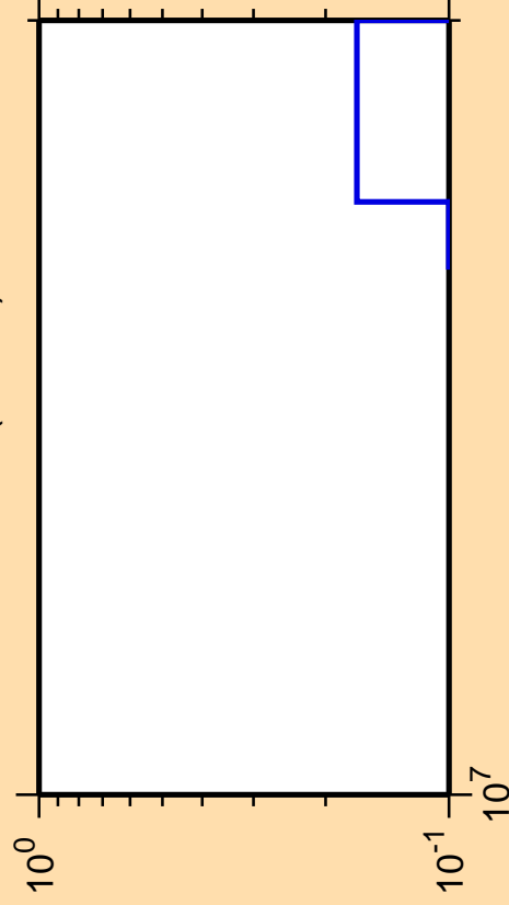
\Delta\sigma/\sigma vs. E for ^{262}\text{Lw} (mt 11)
