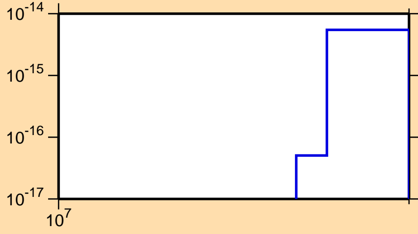
\sigma vs. E for ^{262}\text{Lw} (mt 34)
