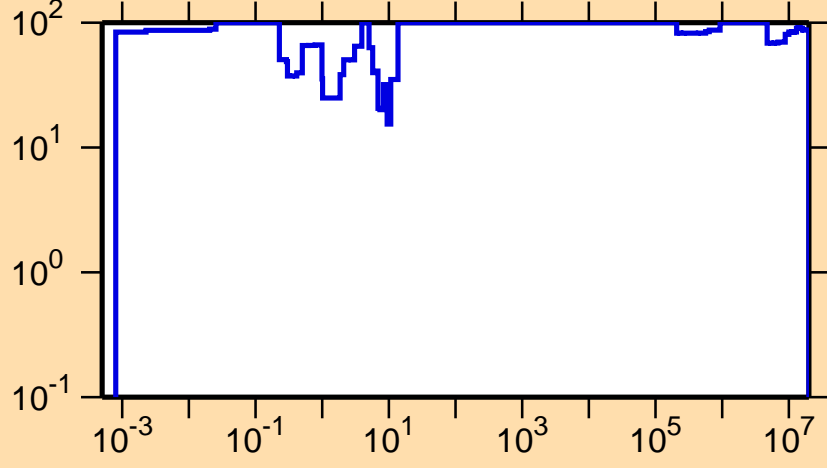
\Delta\sigma/\sigma vs. E for ^{262}\text{Lw}(n,\gamma)
