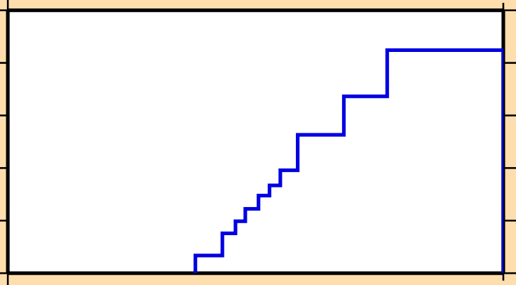
\sigma vs. E for ^{262}\text{Lw}(n,\text{He3})
