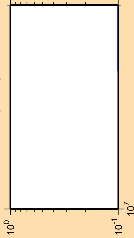
\Delta\sigma/\sigma vs. E for ^{262}\text{Lw} (mt 34)
