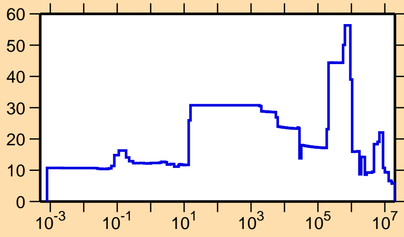
\Delta\sigma/\sigma vs. E for ^{262}\text{Lw}(n,\text{el.})
