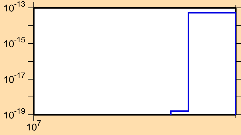
\sigma vs. E for ^{262}\text{Lw} (mt 11)
