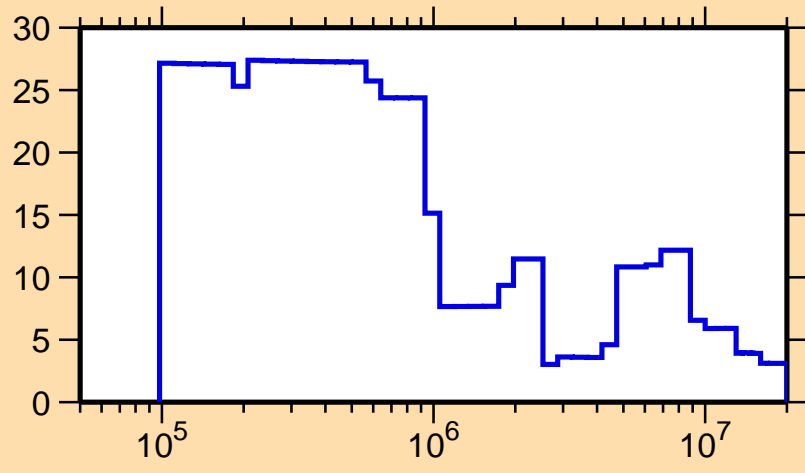
\Delta\sigma/\sigma vs. E for ^{262}\text{Lw}(n, \text{tot.})
