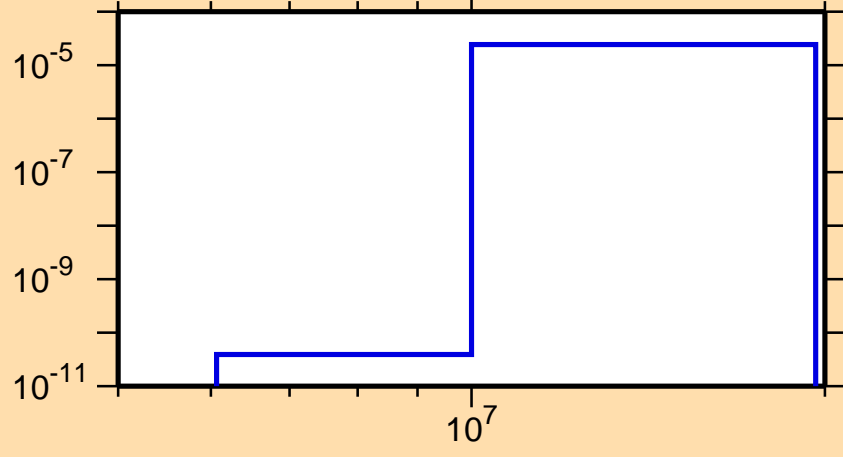
\sigma vs. E for ^{262}\text{Lw}(n,np)
