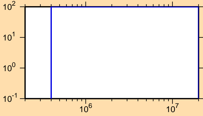
\Delta\sigma/\sigma vs. E for ^{262}\text{Lw}(n,ncont.)
