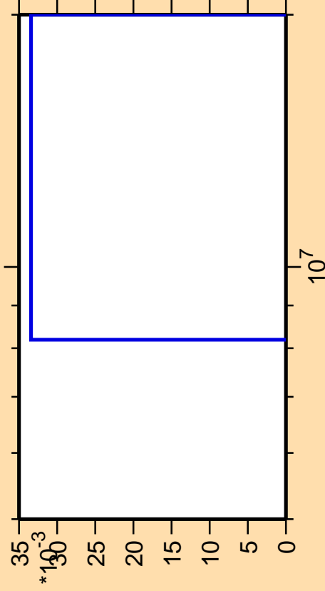
\Delta\sigma/\sigma vs. E for ^{262}\text{Lw}(n,3n\alpha)
