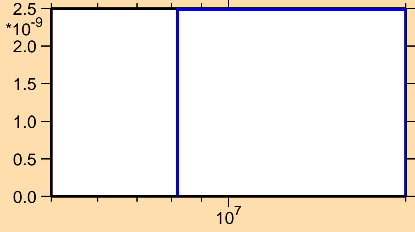
\sigma vs. E for ^{262}\text{Lw}(n,2np)
