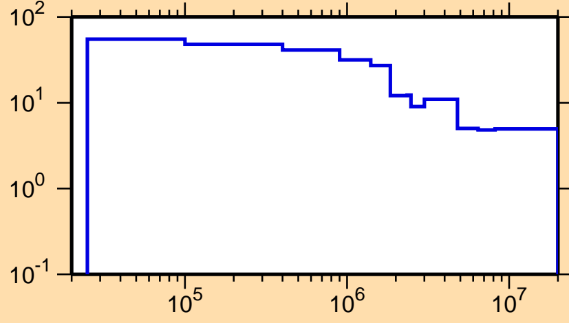
\Delta\sigma/\sigma vs. E for ^{262}\text{Lw}(n,n\text{nonel.})
