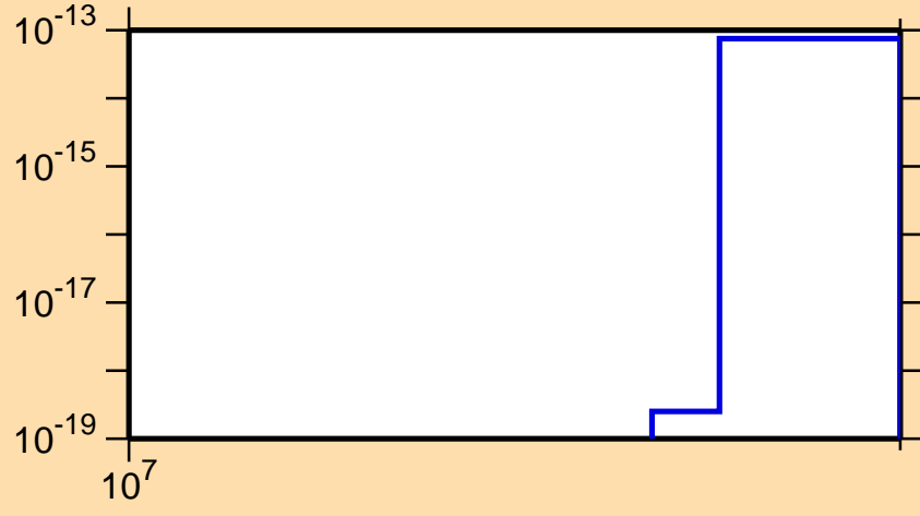
\sigma vs. E for ^{263}\text{Lw} (mt 11)
