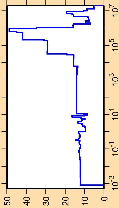
\Delta\sigma/\sigma vs. E for ^{263}\text{Lw}(n,\text{el.})
