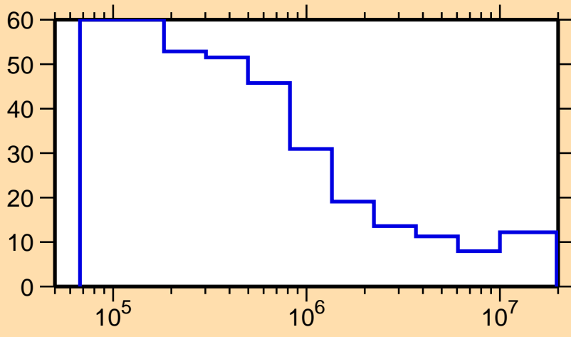
\Delta\sigma/\sigma vs. E for ^{263}\text{Lw}(n,f)
