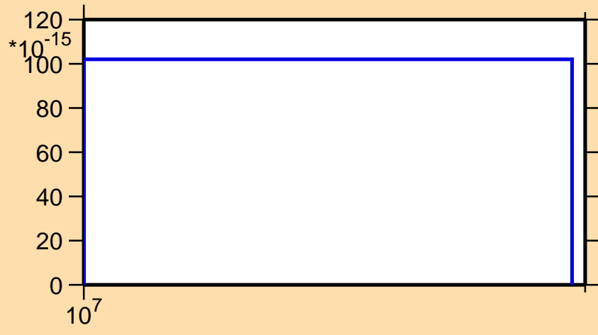
\sigma vs. E for ^{263}\text{Lw}(n,\text{He3})
