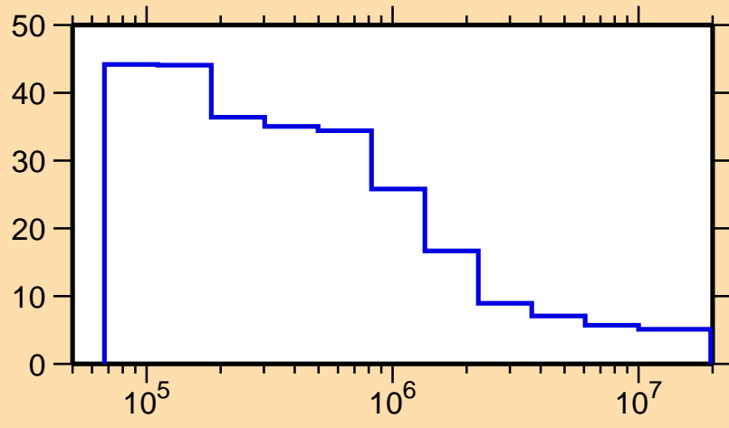
\Delta\sigma/\sigma vs. E for ^{263}\text{Lw}(n,\text{nonel.})
