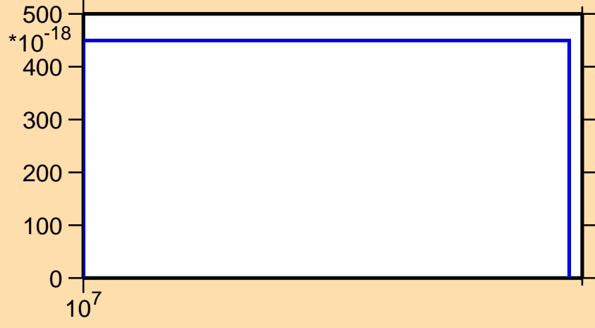
\sigma vs. E for ^{263}\text{Lw}(\text{mt 11})
