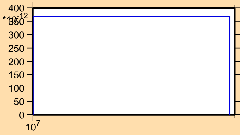
\sigma vs. E for ^{263}\text{Lw}(n,nd)
