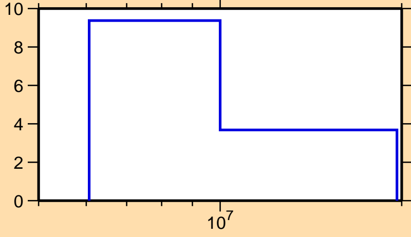
\Delta\sigma/\sigma vs. E for ^{263}\text{Lw}(n,\text{tot.})
