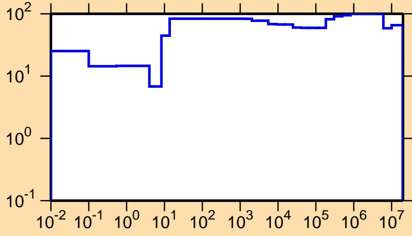
\Delta\sigma/\sigma vs. E for ^{263}\text{Lw}(n,\gamma)
