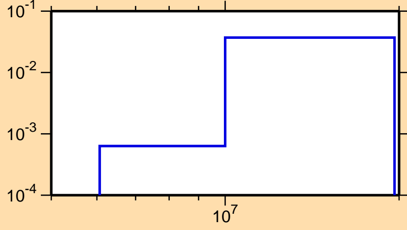
\sigma vs. E for ^{263}\text{Lw}(n,2n)
