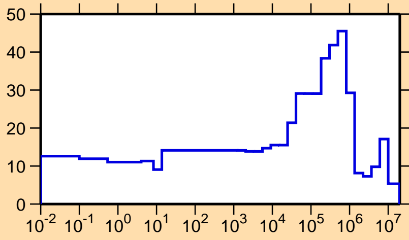
\Delta\sigma/\sigma vs. E for ^{263}\text{Lw}(n,\text{el.})
