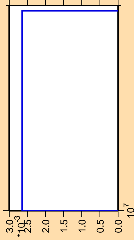
\Delta\sigma/\sigma vs. E for ^{263}\text{Lw}(\text{mt 11})
