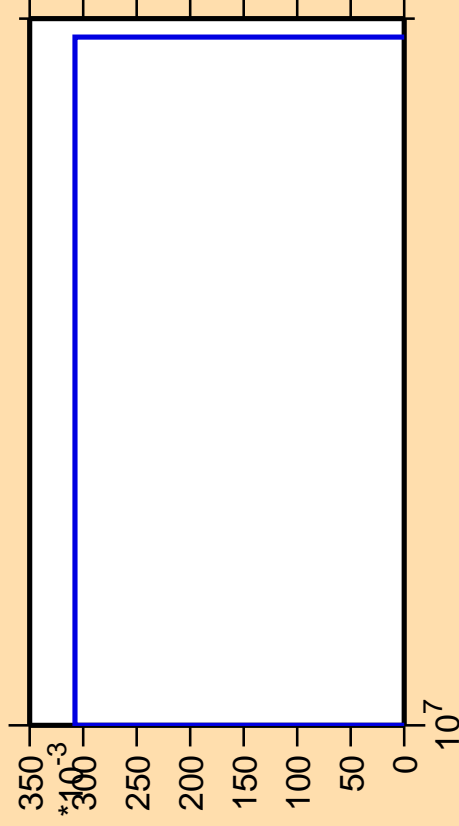
\Delta\sigma/\sigma vs. E for ^{263}\text{Lw}(n,\text{He3})
