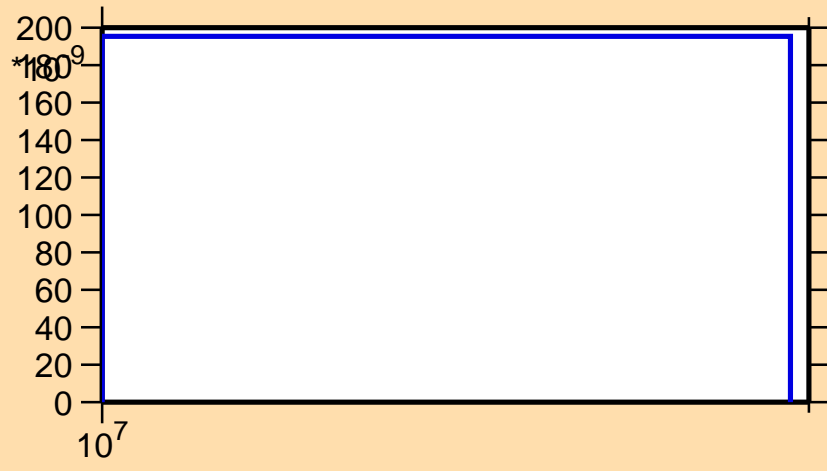
\sigma vs. E for ^{263}\text{Lw}(n,nt)
