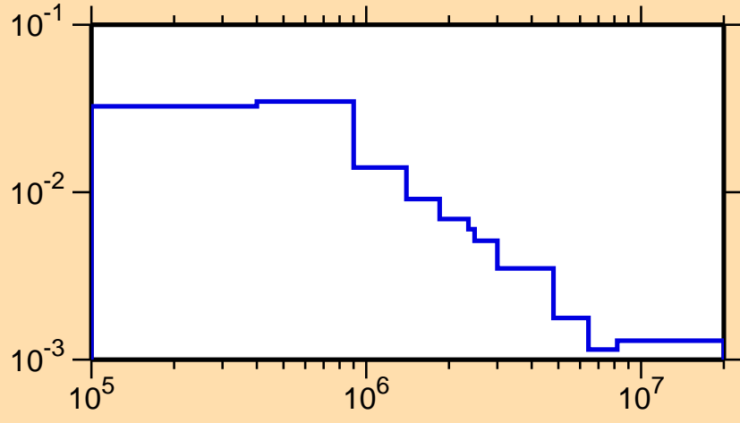
\sigma vs. E for ^{263}\text{Lw}(n,n\text{cont.})
