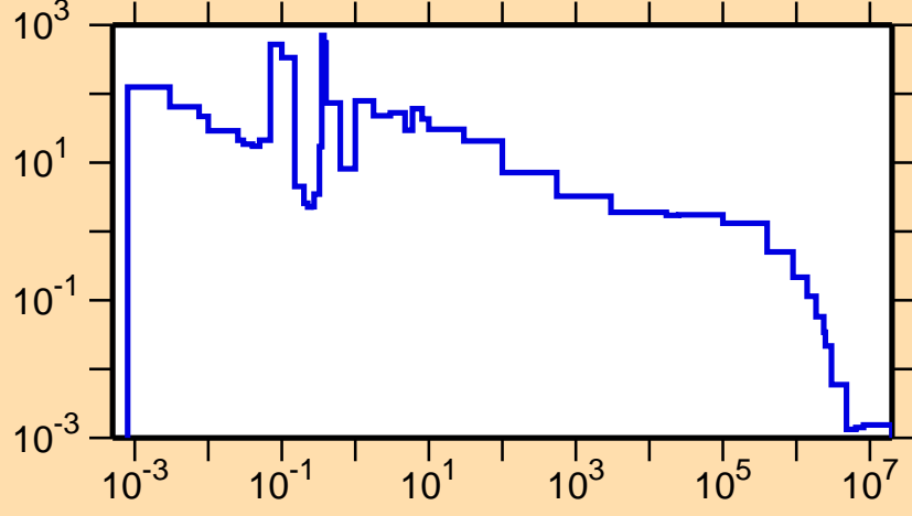
\sigma vs. E for ^{263}\text{Lw}(n,\gamma)
