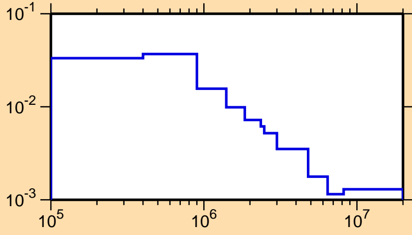
\sigma vs. E for ^{263}\text{Lw}(n,\text{inel.})
