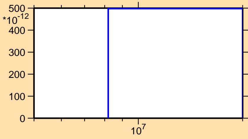
\sigma vs. E for ^{263}\text{Lw}(n,2n\alpha)
