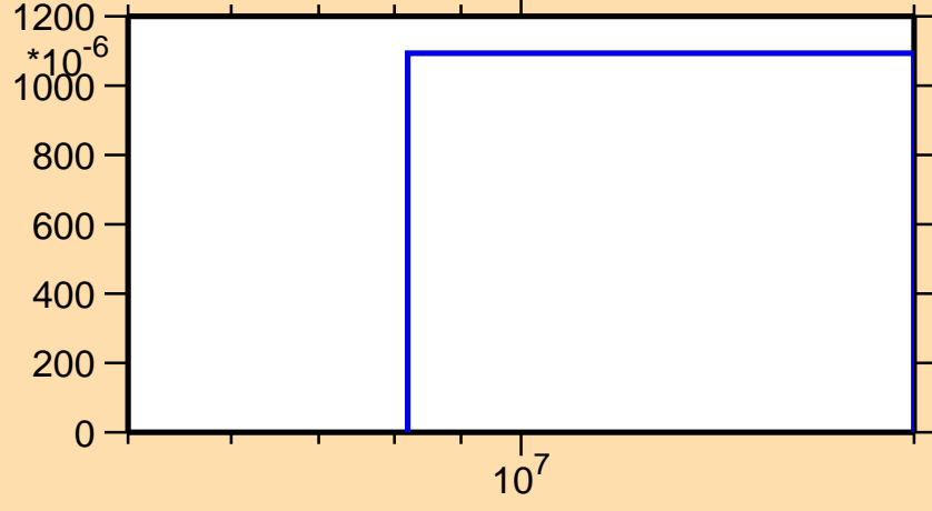
\sigma vs. E for ^{263}\text{Lw}(n,3n)
