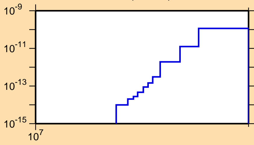
\sigma vs. E for ^{264}\text{Lw}(n,\text{He3})
