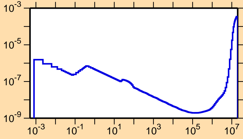
\sigma vs. E for ^{264}\text{Lw}(n,\alpha)
