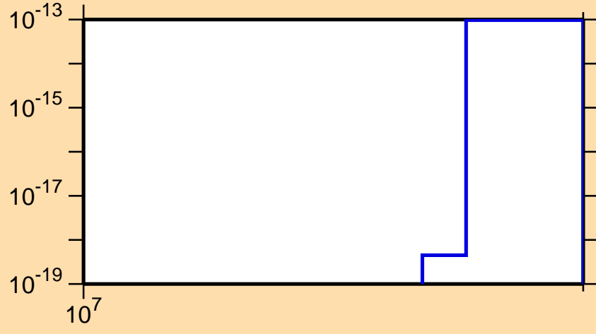
\sigma vs. E for ^{264}\text{Lw}(\text{mt } 11)
