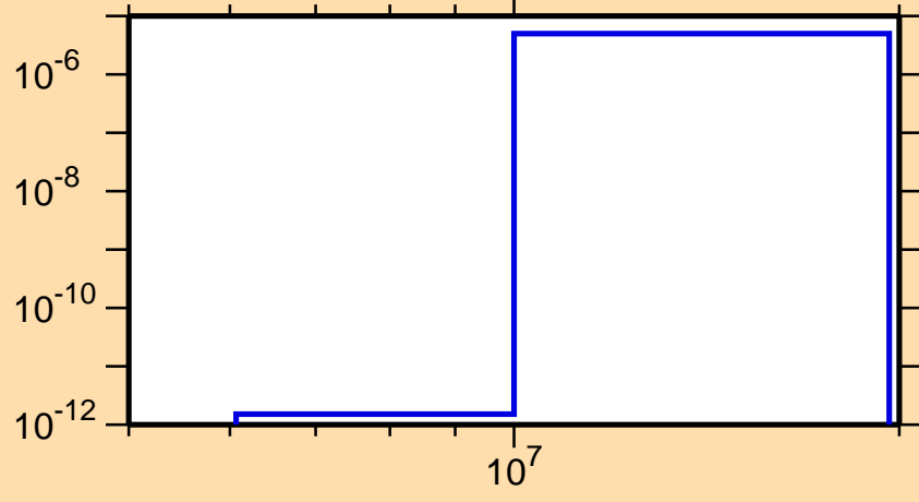
\sigma vs. E for ^{264}\text{Lw}(n,np)
