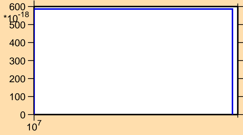
\sigma vs. E for ^{264}\text{Lw}(\text{mt } 11)
