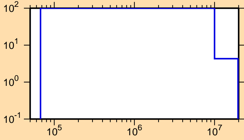
\Delta\sigma/\sigma vs. E for ^{264}\text{Lw}(n,n_1)
