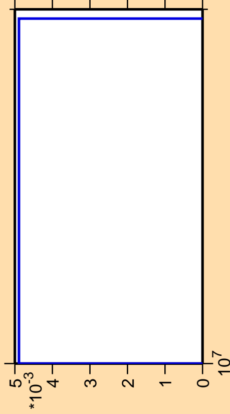
\Delta\sigma/\sigma vs. E for ^{264}\text{Lw}(\text{mt } 11)
