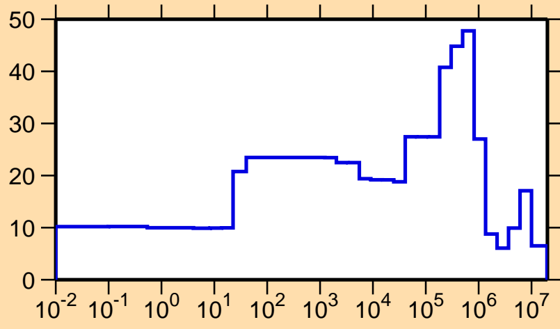
\Delta\sigma/\sigma vs. E for ^{264}\text{Lw}(n,\text{el.})
