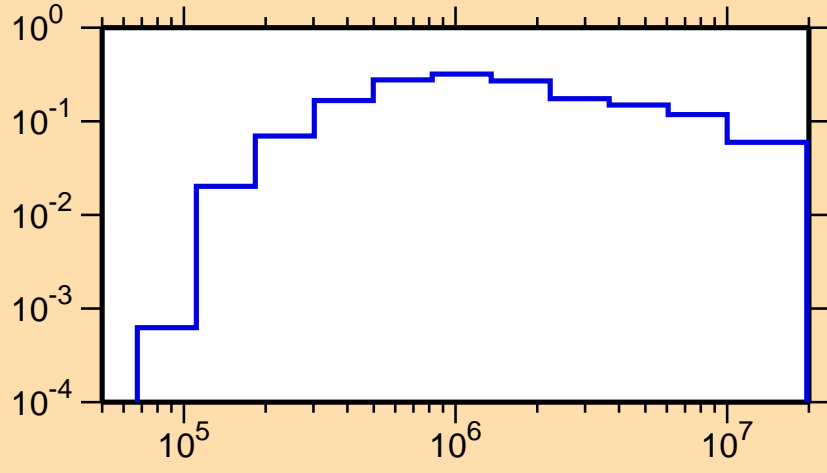
\sigma vs. E for ^{264}\text{Lw}(n,n\text{cont.})
