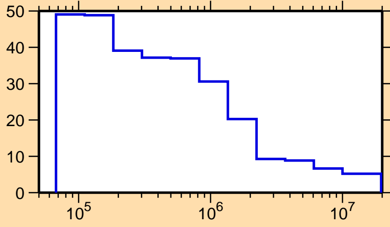
\Delta\sigma/\sigma vs. E for ^{264}\text{Lw}(n,\text{nonel.})
