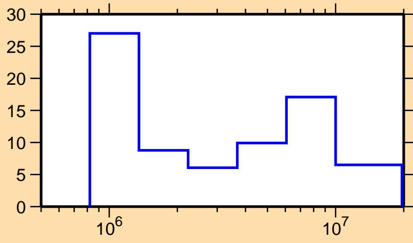
\Delta\sigma/\sigma vs. E for ^{264}\text{Lw}(n,el.)
