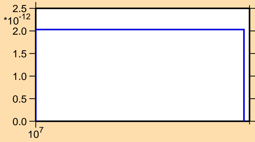
\sigma vs. E for ^{264}\text{Lw}(n,\text{He3})
