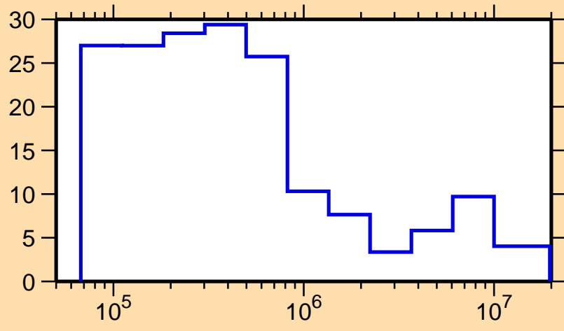
\Delta\sigma/\sigma vs. E for ^{264}\text{Lw}(n,\text{tot.})
