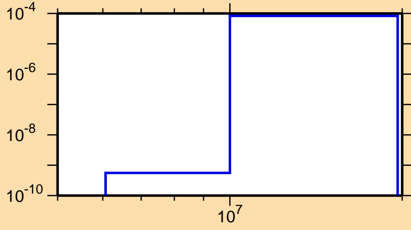
\sigma vs. E for ^{264}\text{Lw}(n,d)
