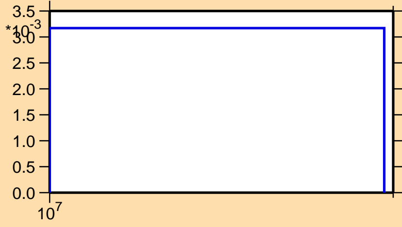
\sigma vs. E for ^{264}\text{Lw}(n,3n)
