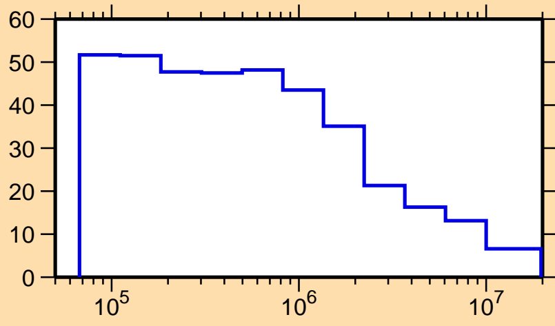
\Delta\sigma/\sigma vs. E for ^{264}\text{Lw}(n,f)
