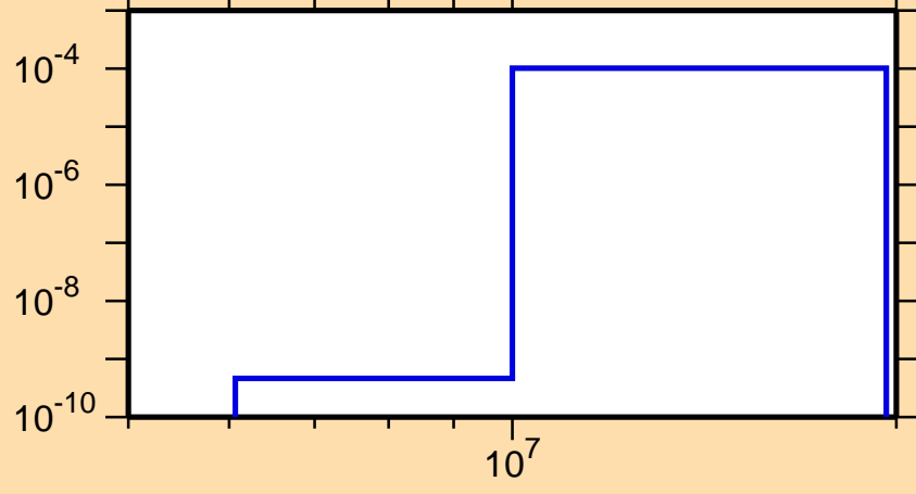
\sigma vs. E for ^{264}\text{Lw}(n,t)
