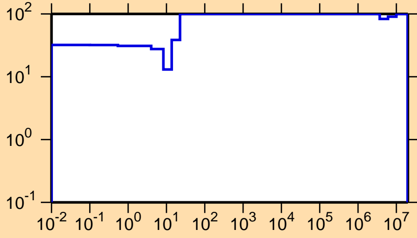
\Delta\sigma/\sigma vs. E for ^{264}\text{Lw}(n,\gamma)
