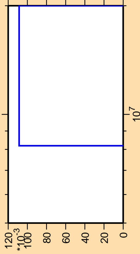
\Delta\sigma/\sigma vs. E for ^{264}\text{Lw}(n,3n\alpha)
