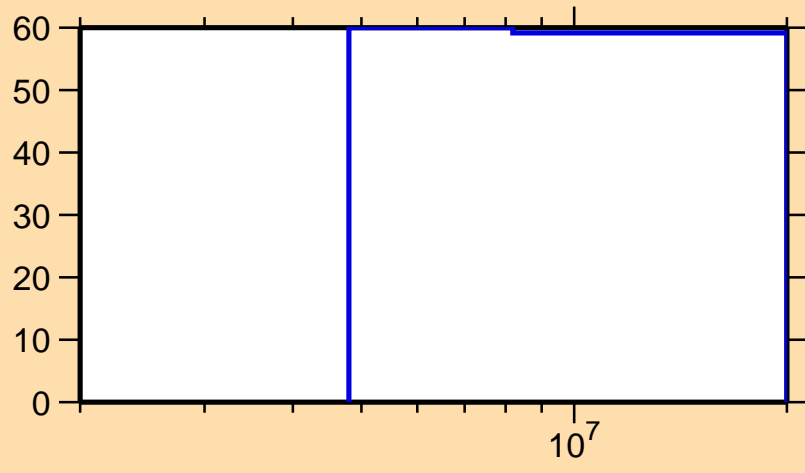
\Delta\sigma/\sigma vs. E for ^{264}\text{Lw}(n,\text{inel.})
