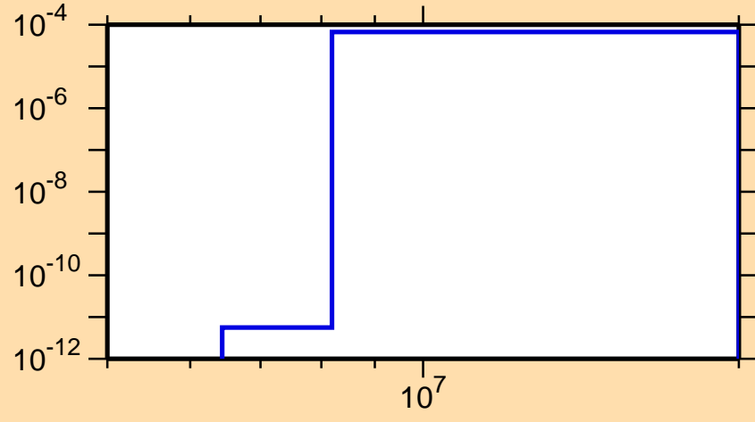
\sigma vs. E for ^{264}\text{Lw}(n,d)
