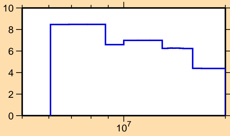
\Delta\sigma/\sigma vs. E for ^{265}\text{Lw}(n,\text{tot.})
