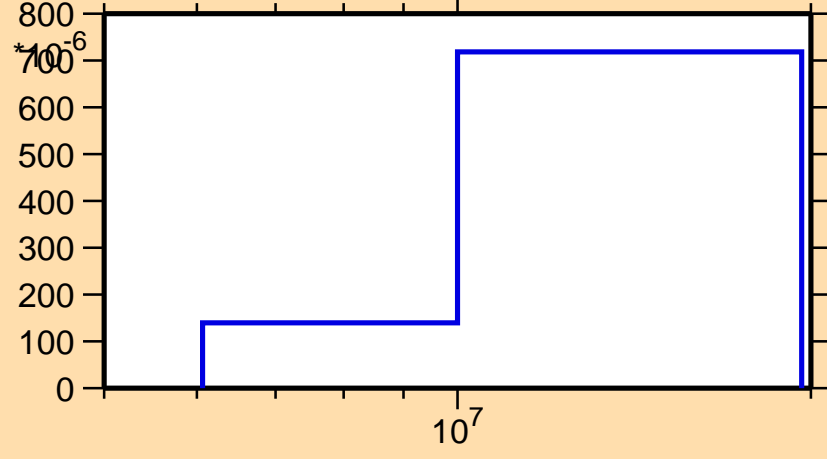
\sigma vs. E for ^{265}\text{Lw}(n,2n)
