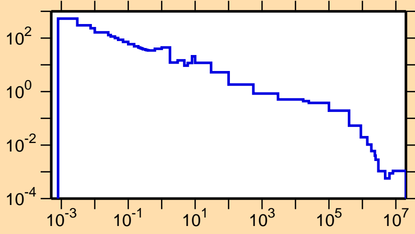
\sigma vs. E for ^{265}\text{Lw}(n,\gamma)
