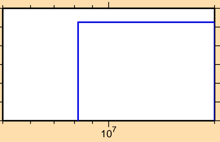
\sigma vs. E for ^{265}\text{Lw}(n,\text{He3})
