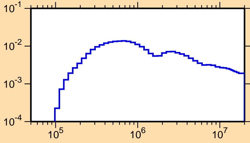
\sigma vs. E for ^{266}\text{Lw}(n,\text{inel.})
