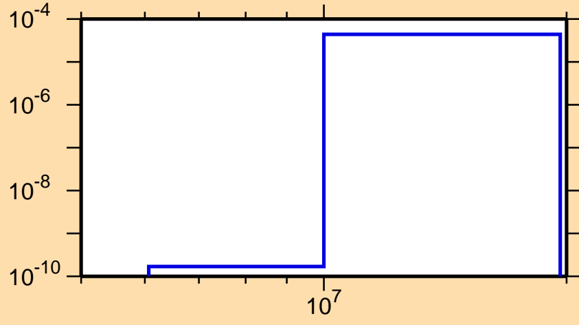
\sigma vs. E for ^{266}\text{Lw}(n,d)
