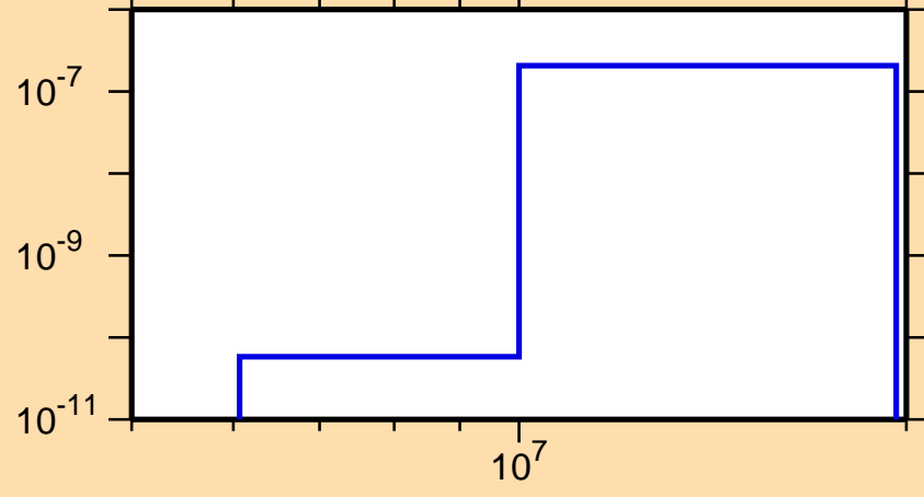
\sigma vs. E for ^{266}\text{Lw}(n,t)
