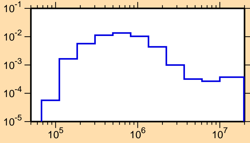
\sigma vs. E for ^{266}\text{Lw}(n,n\text{cont.})
