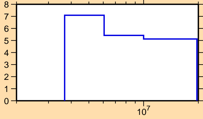
\Delta\sigma/\sigma vs. E for ^{266}\text{Lw}(n,\text{nonel.})
