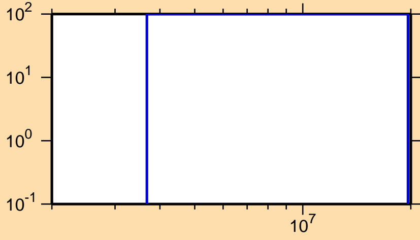
\Delta\sigma/\sigma vs. E for ^{266}\text{Lw}(n, 2n)
