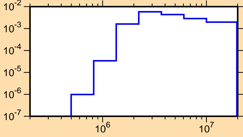
\sigma vs. E for ^{266}\text{Lw}(n,n_1)
