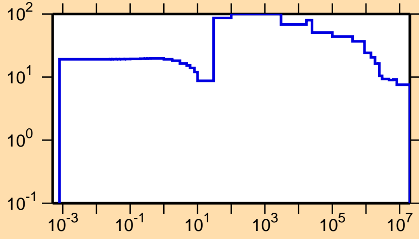
\Delta\sigma/\sigma vs. E for ^{266}\text{Lw}(n,f)
