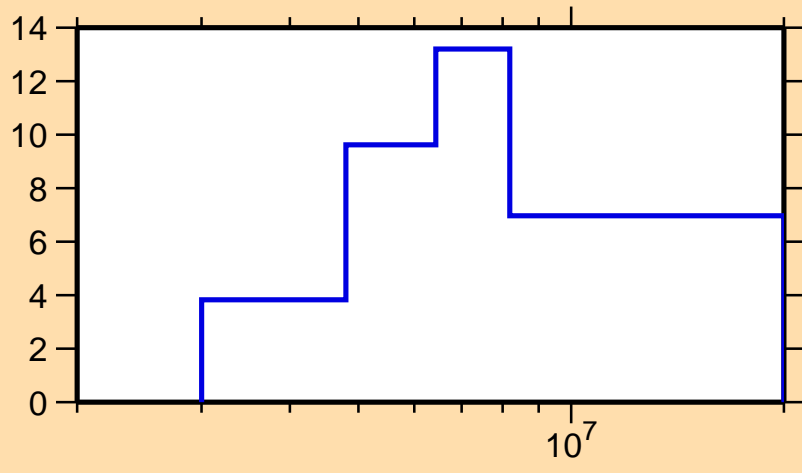
\Delta\sigma/\sigma vs. E for ^{266}\text{Lw}(n,\text{tot.})
