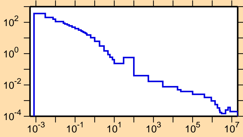
\sigma vs. E for ^{266}\text{Lw}(n,\gamma)
