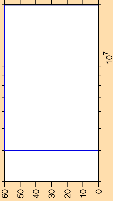
\Delta\sigma/\sigma vs. E for ^{266}\text{Lw}(n, n_{\text{cont}}) .
