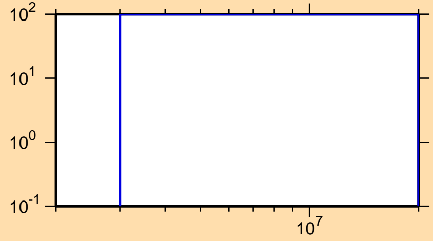
\Delta\sigma/\sigma vs. E for ^{266}\text{Lw}(n, 2n)
