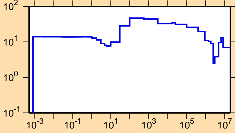
\Delta\sigma/\sigma vs. E for ^{266}\text{Lw}(n,\text{tot.})
