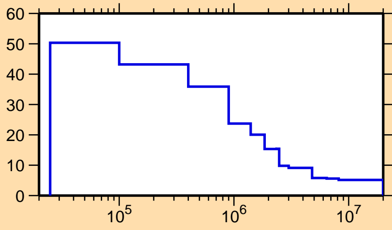
\Delta\sigma/\sigma vs. E for ^{266}\text{Lw}(n,\text{nonel.})
