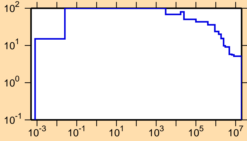
\Delta\sigma/\sigma vs. E for ^{266}\text{Lw}(n,\text{nonel.})
