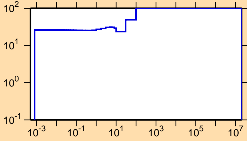
\Delta\sigma/\sigma vs. E for ^{266}\text{Lw}(n,\gamma)
