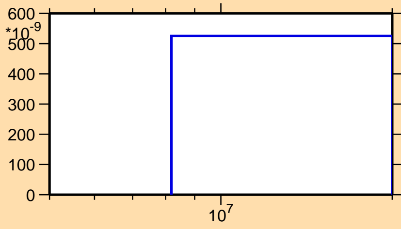
\sigma vs. E for ^{266}\text{Lw}(n,np)
