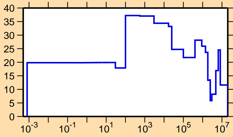
\Delta\sigma/\sigma vs. E for ^{266}\text{Lw}(n,\text{el.})
