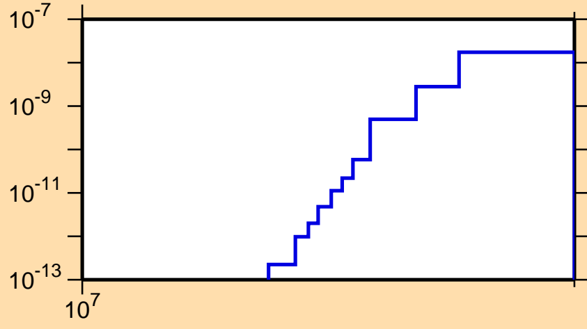
\sigma vs. E for ^{154}\text{Lu}(n,2n\alpha)
