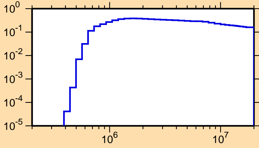
\sigma vs. E for ^{154}\text{Lu}(n,\text{inel.})
