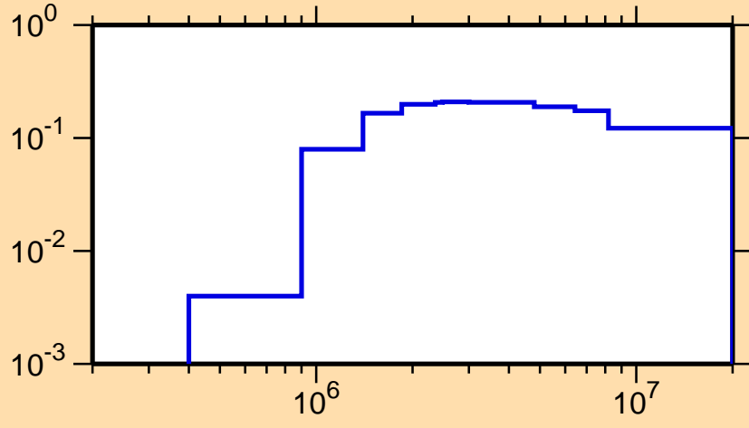
\sigma vs. E for ^{154}\text{Lu}(n,n\text{cont.})
