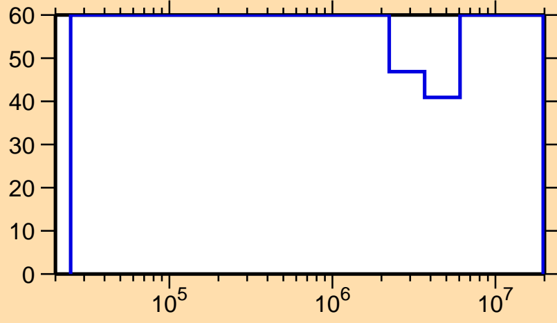
\Delta\sigma/\sigma vs. E for ^{157}\text{Lu}(n,n_1)
