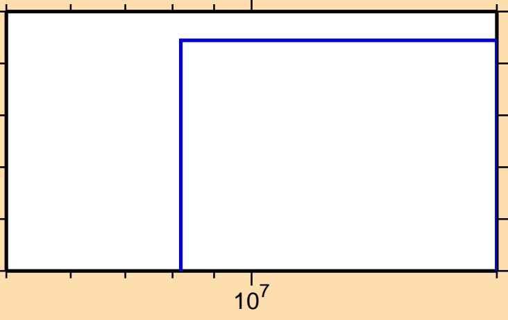
\sigma vs. E for ^{157}\text{Lu}(n,nd)
