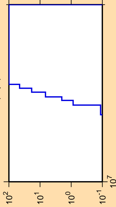
\Delta\sigma/\sigma vs. E for ^{157}\text{Lu}(n,pt)
