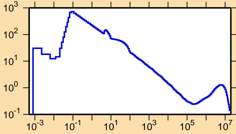
\sigma vs. E for ^{157}\text{Lu}(n,p)
