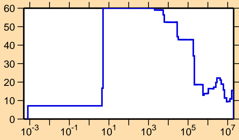
\Delta\sigma/\sigma vs. E for ^{157}\text{Lu}(n,el.)
