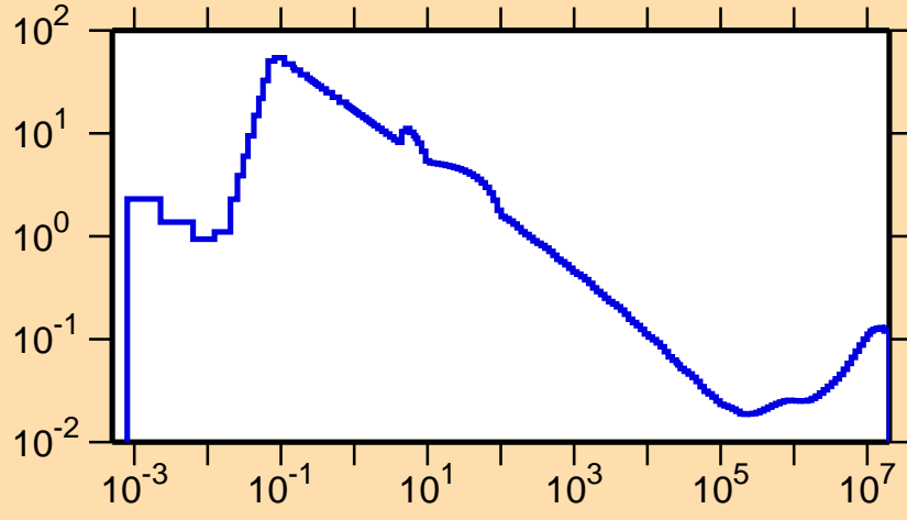
\sigma vs. E for ^{157}\text{Lu}(n,\alpha)
