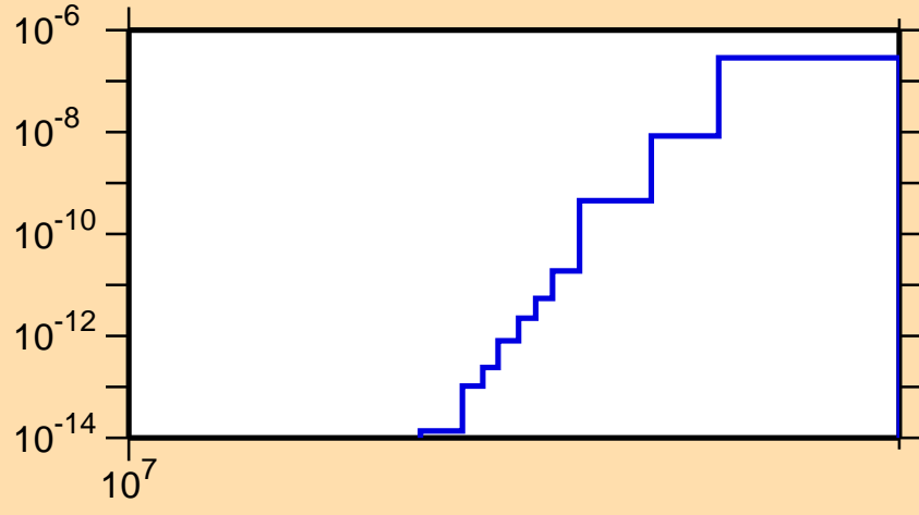
\sigma vs. E for ^{157}\text{Lu}(n,pt)
